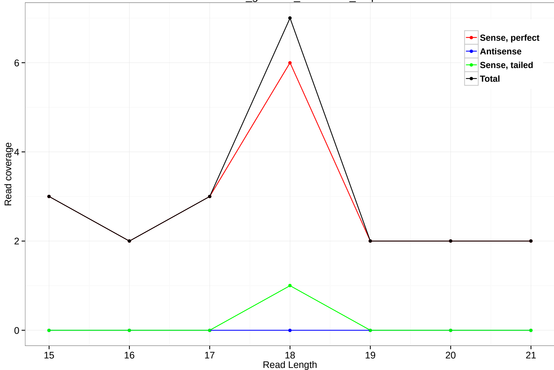
rheMac3_genscan_chr1.3178_0.5p
