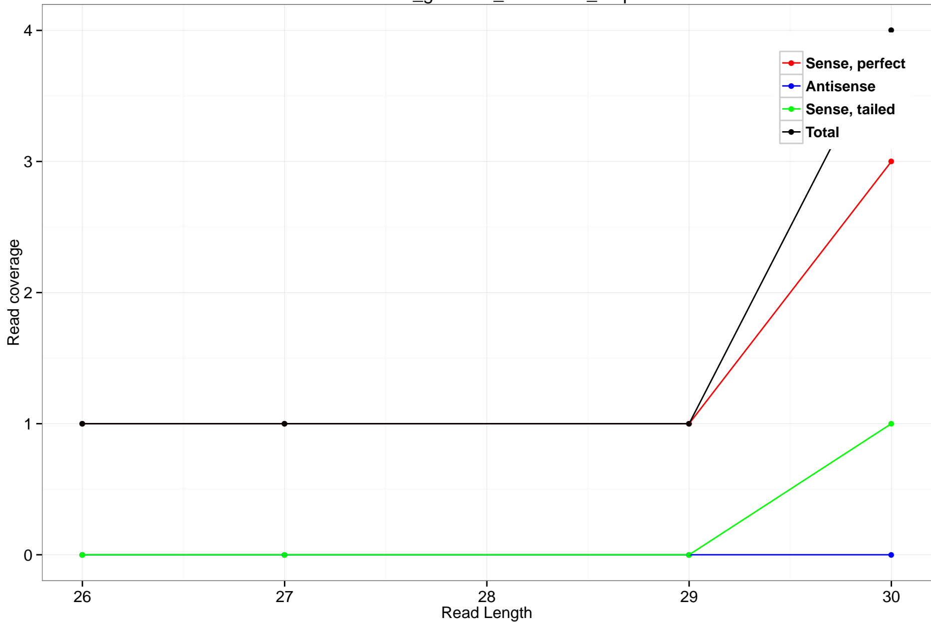
rheMac3_genscan_chr1.3013_0.3p
