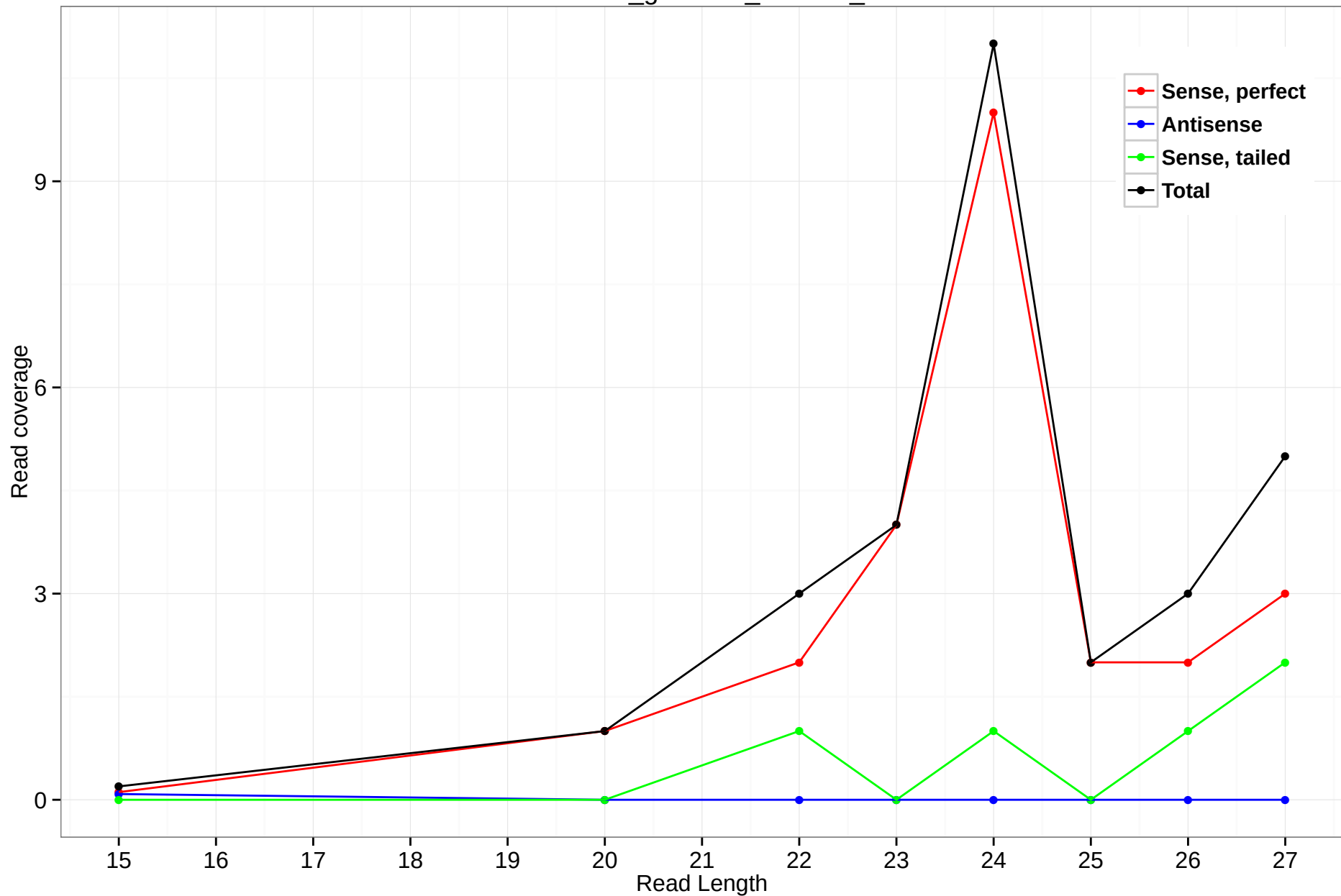
rheMac3_genscan_chr1.29_9
