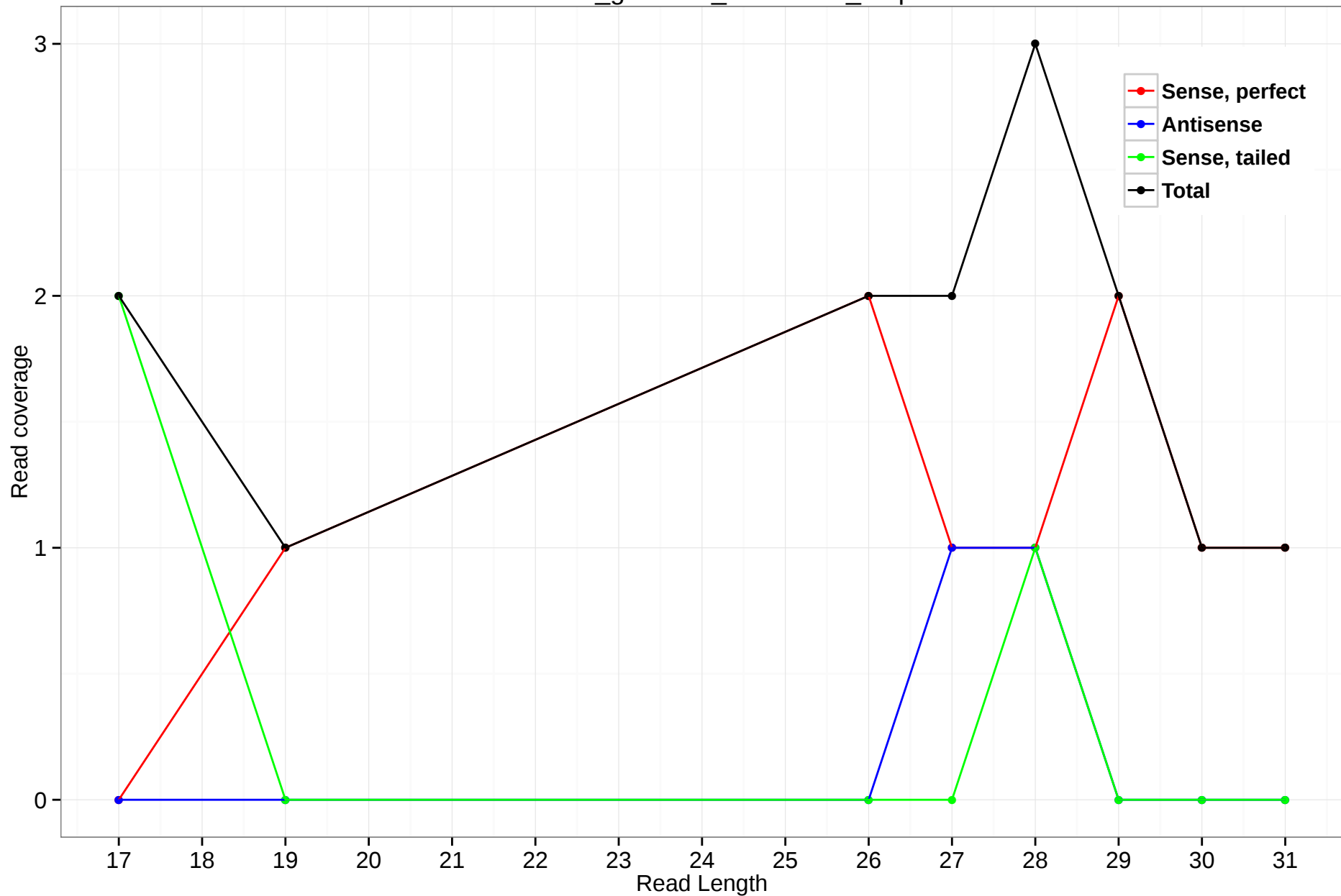
rheMac3_genscan_chr1.2987_9.3p
