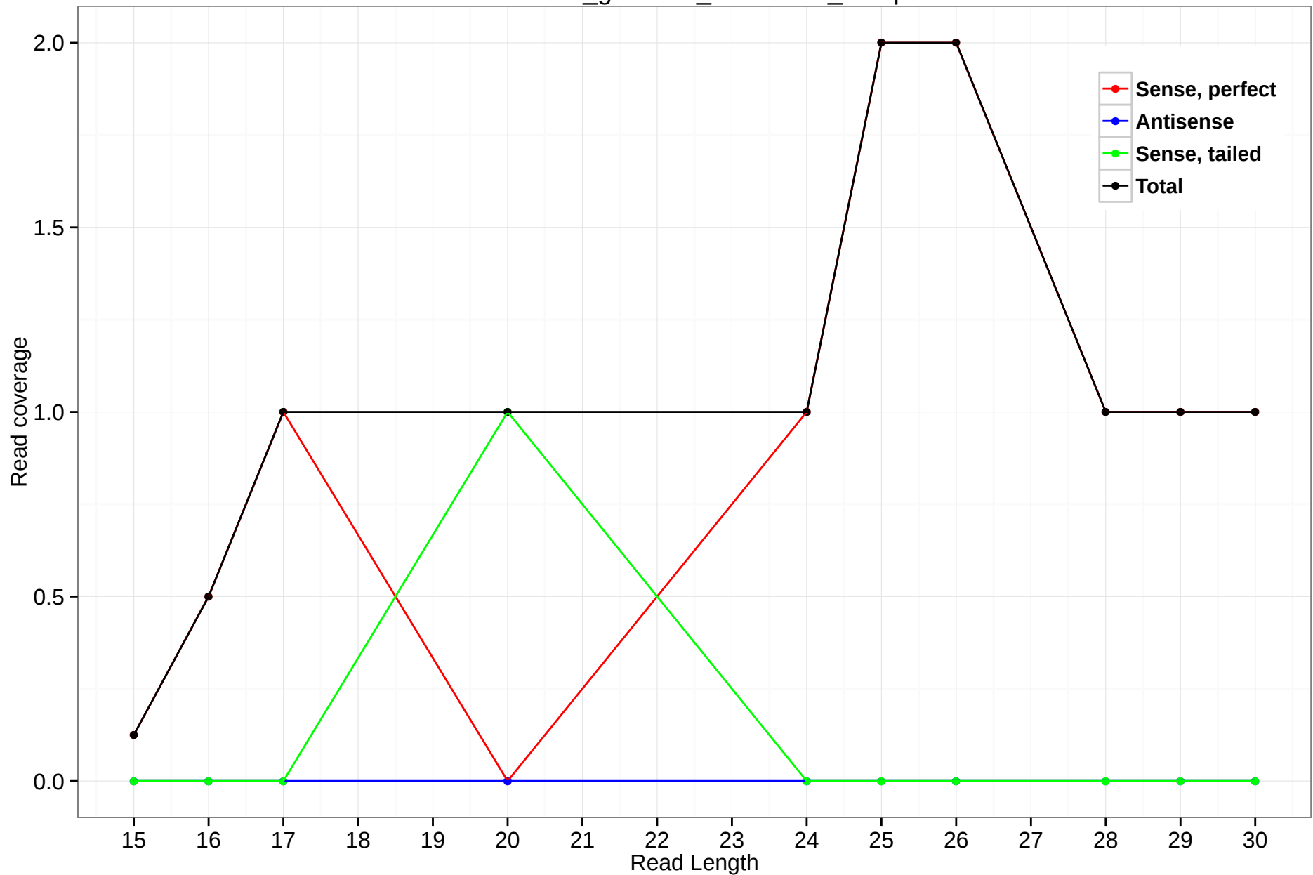
rheMac3_genscan_chr1.2987_62.5p
