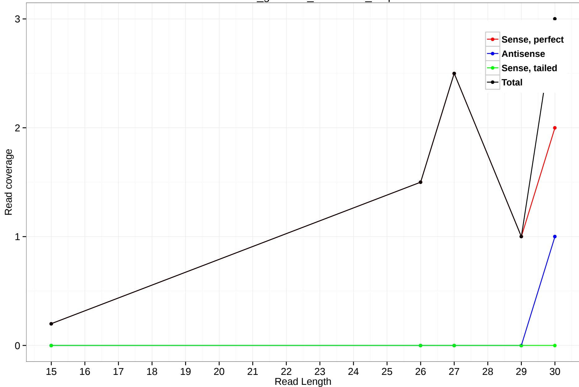
rheMac3_genscan_chr1.2940_4.5p
