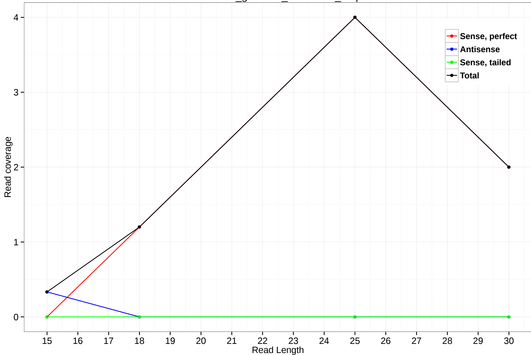
rheMac3_genscan_chr1.2903_3.5p
