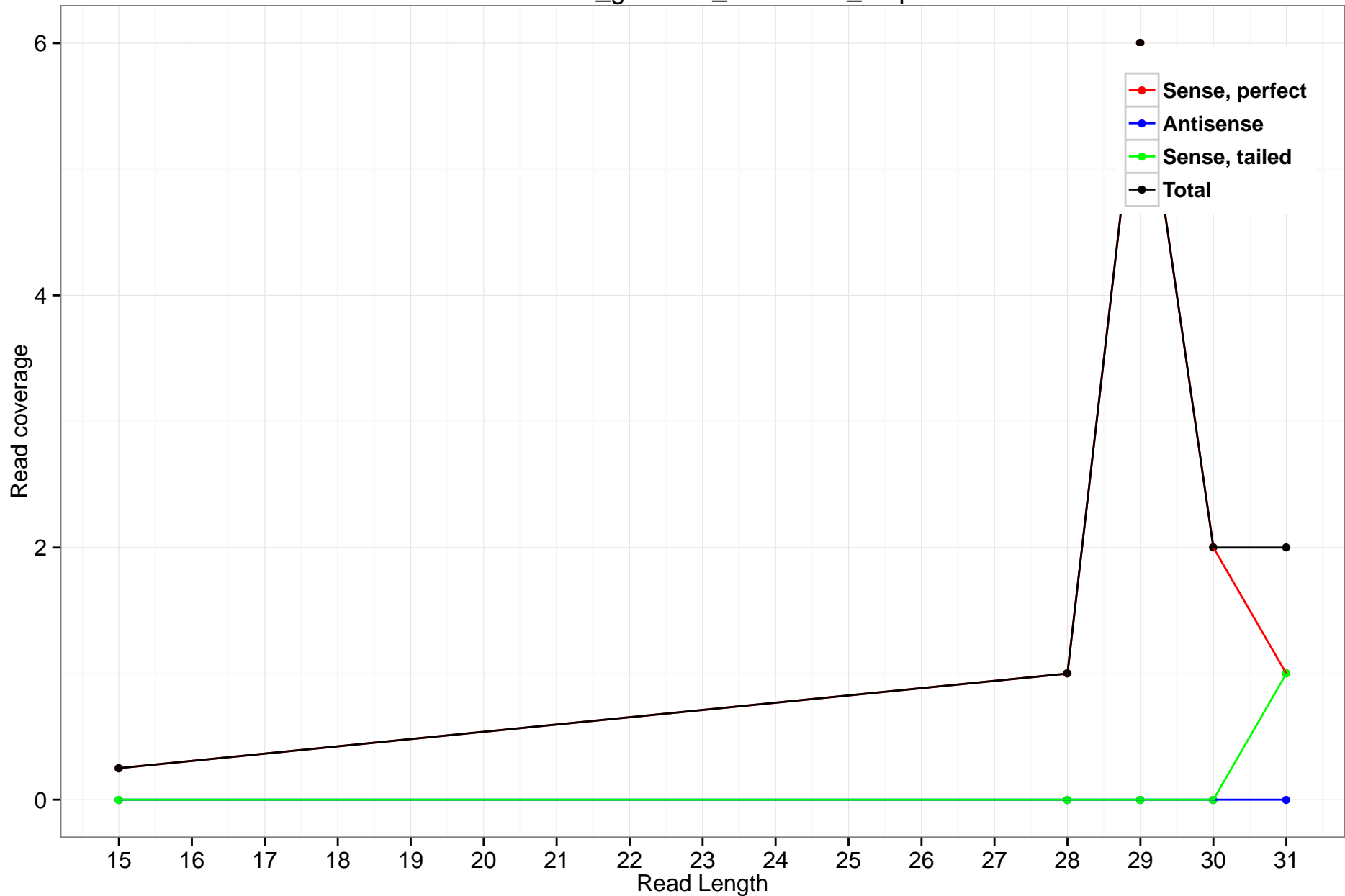
rheMac3_genscan_chr1.2903_2.3p
