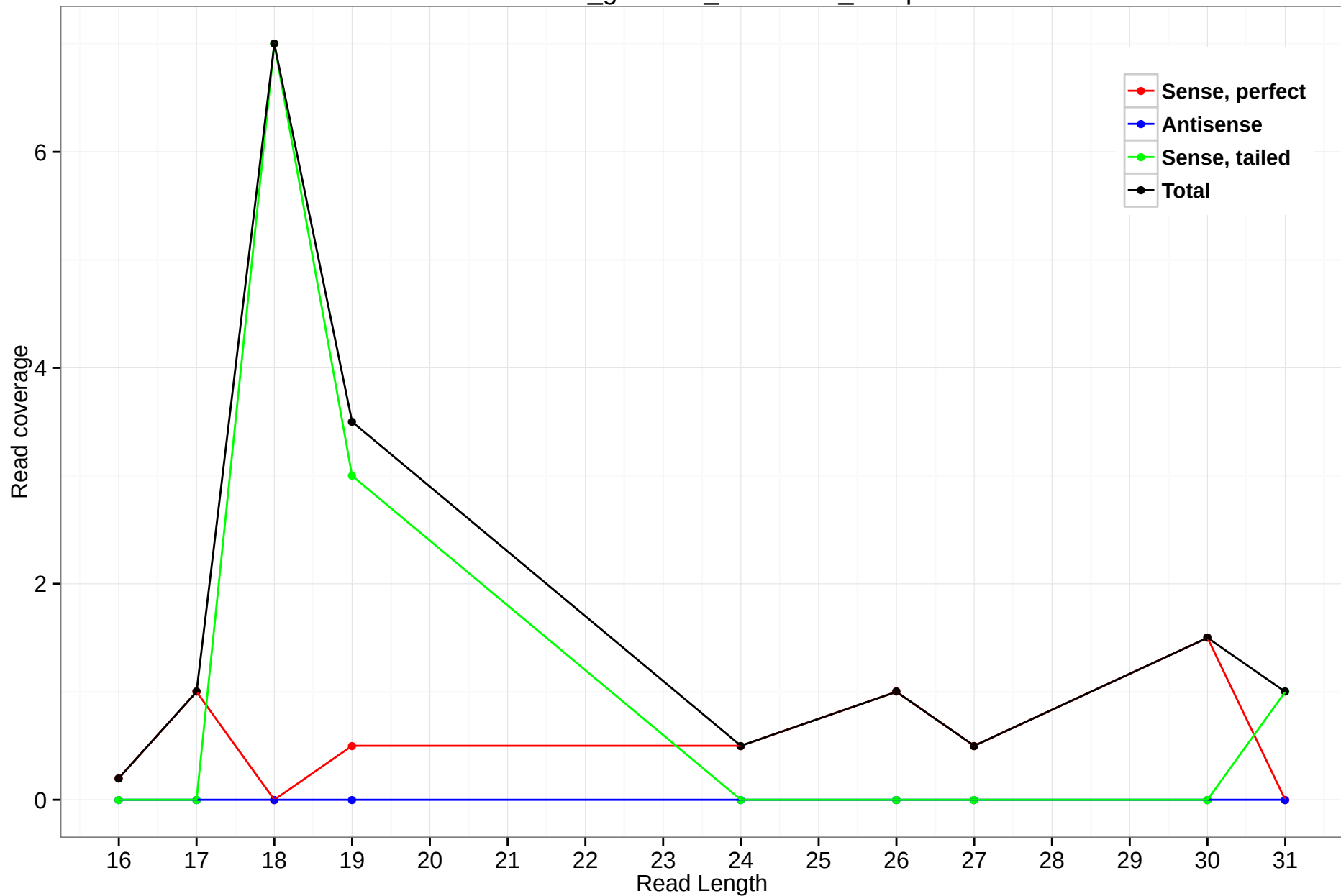
rheMac3_genscan_chr1.2897_36.3p
