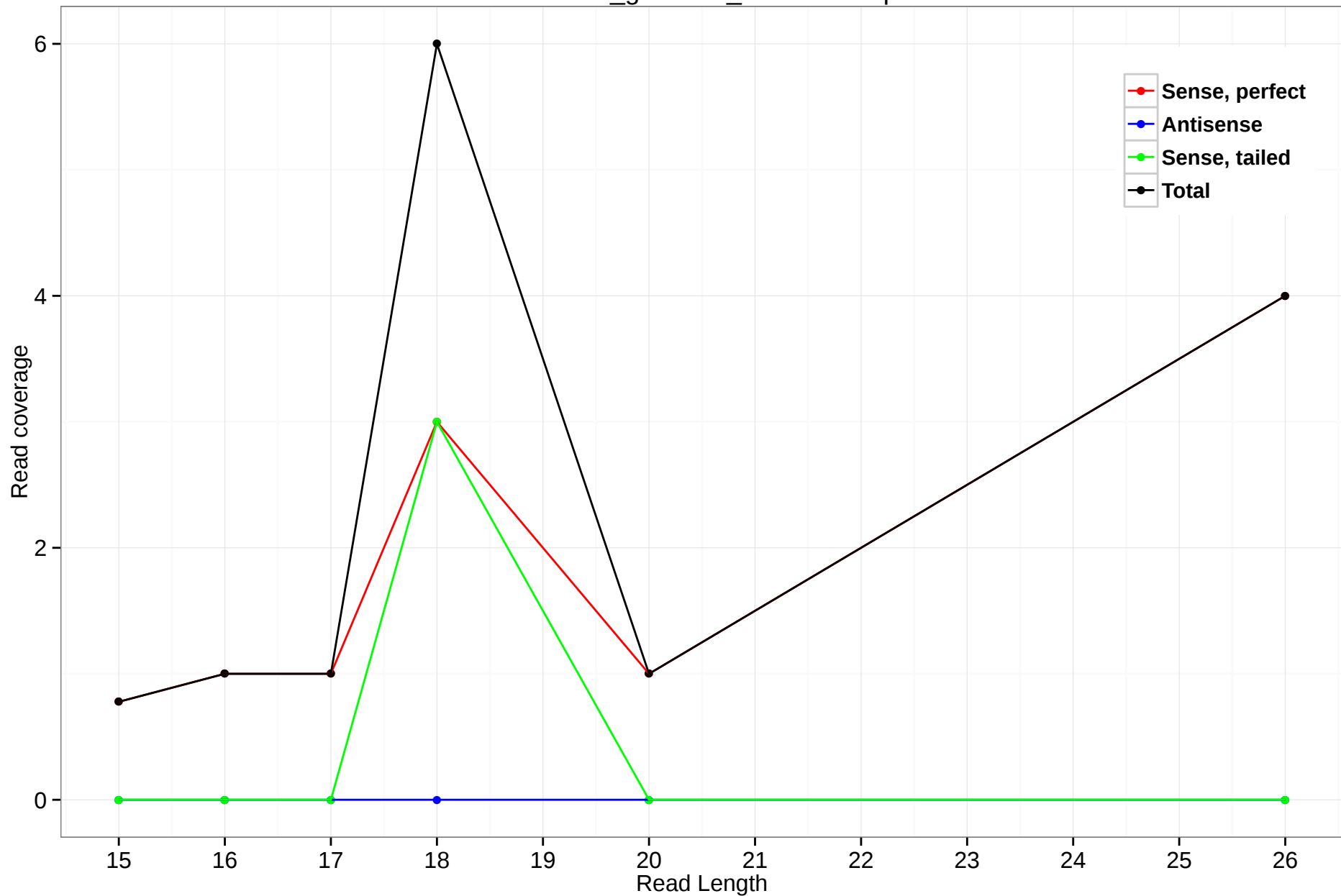
rheMac3_genscan_chr1.2895.5p
