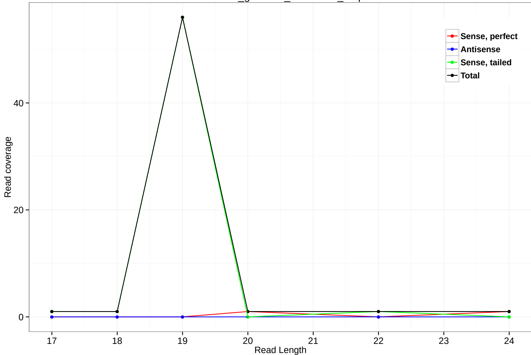
rheMac3_genscan_chr1.2883_0.3p
