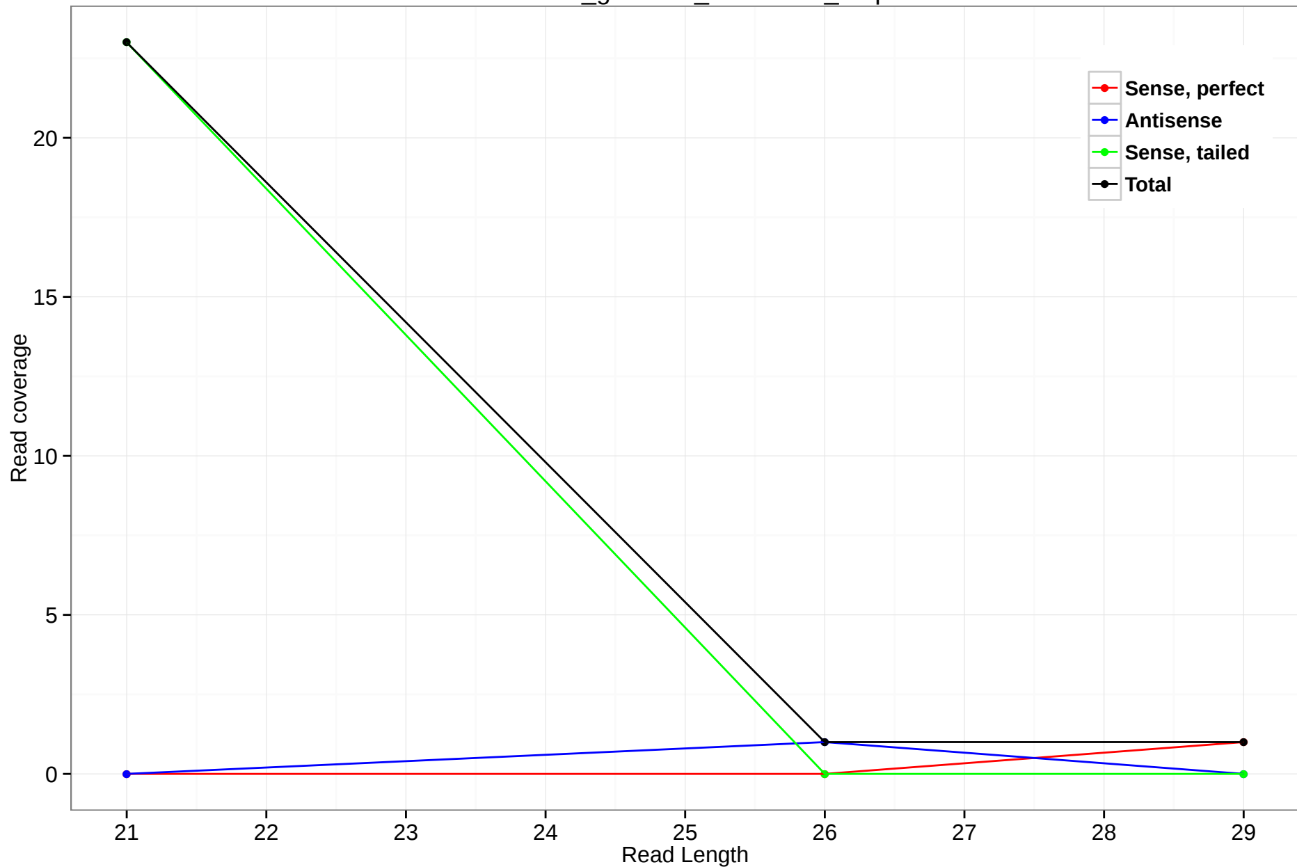
rheMac3_genscan_chr1.2834_7.5p
