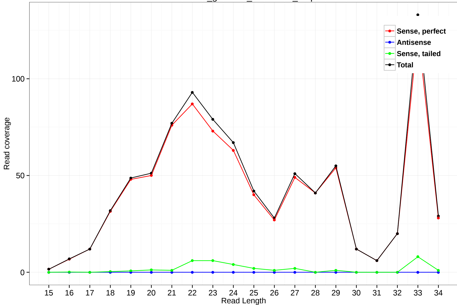
rheMac3_genscan_chr1.2785_5.3p
