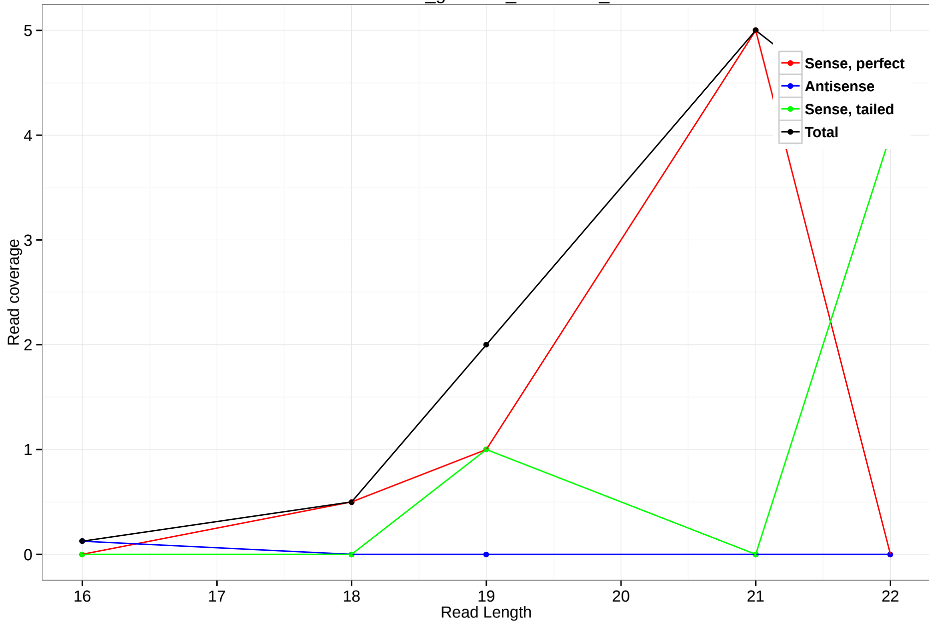
rheMac3_genscan_chr1.2785_0
