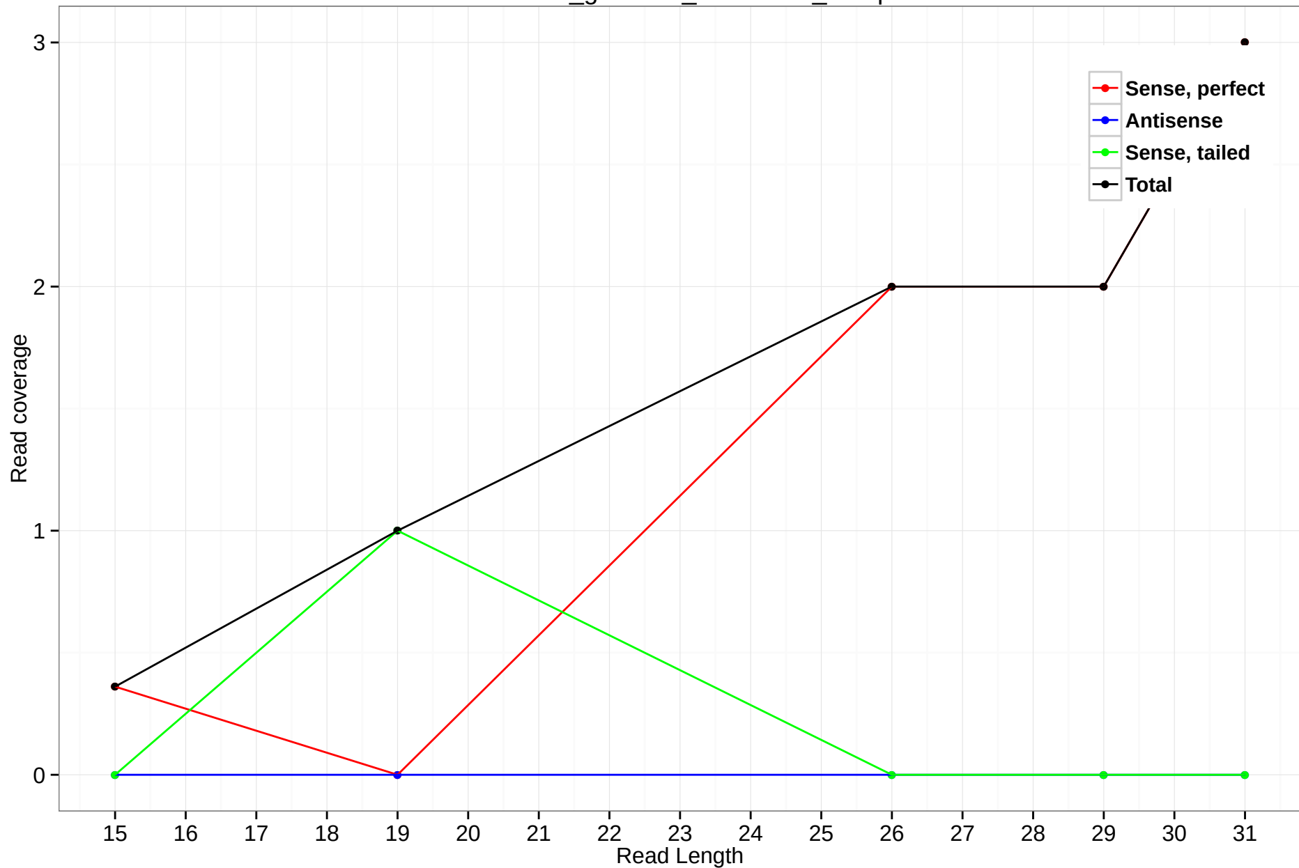
rheMac3_genscan_chr1.2759_12.3p
