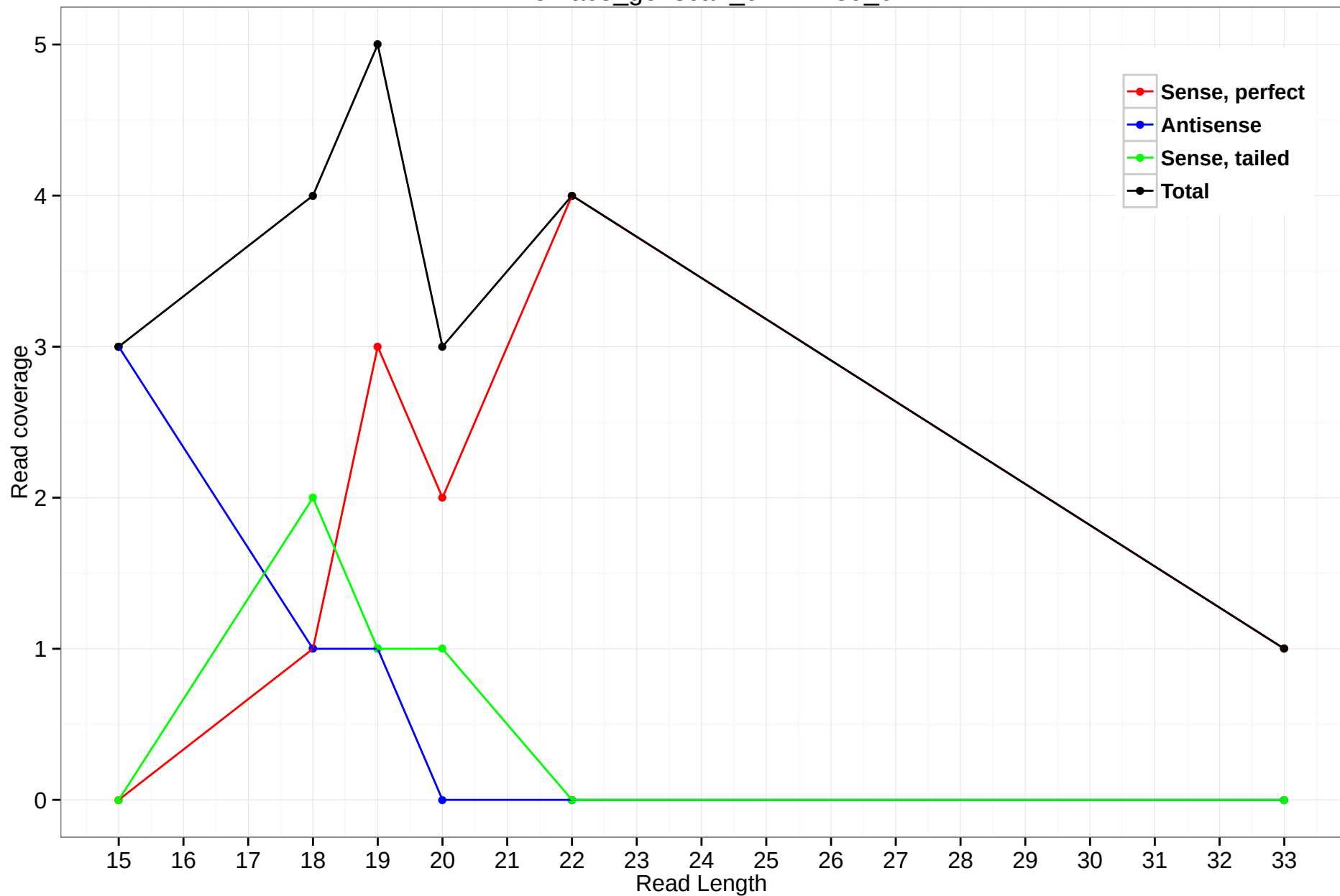
rheMac3_genscan_chr1.2759_0
