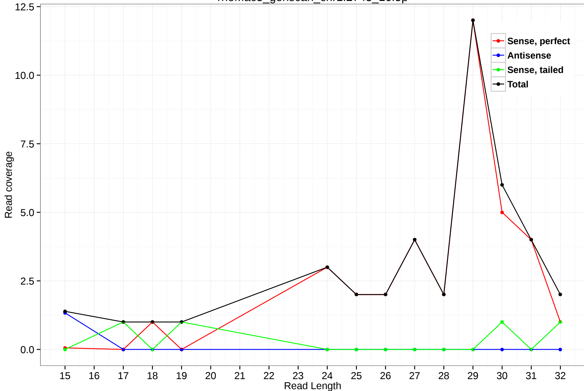
rheMac3_genscan_chr1.2743_16.5p
