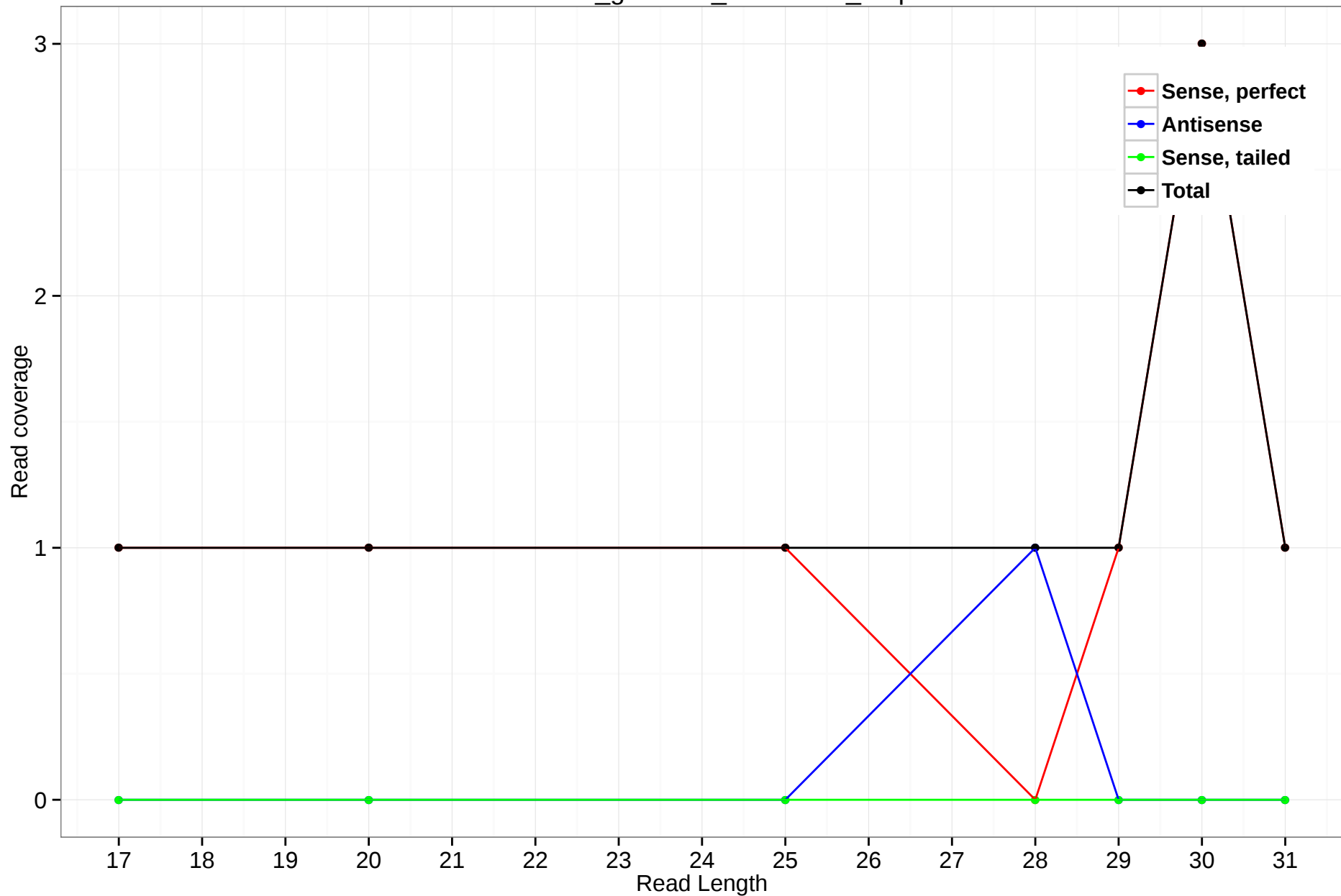
rheMac3_genscan_chr1.2740_3.3p
