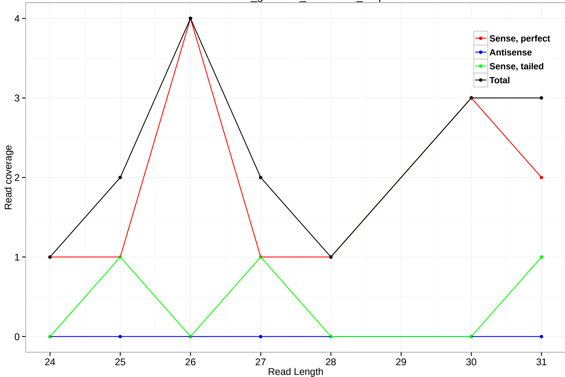
rheMac3_genscan_chr1.2738_6.5p
