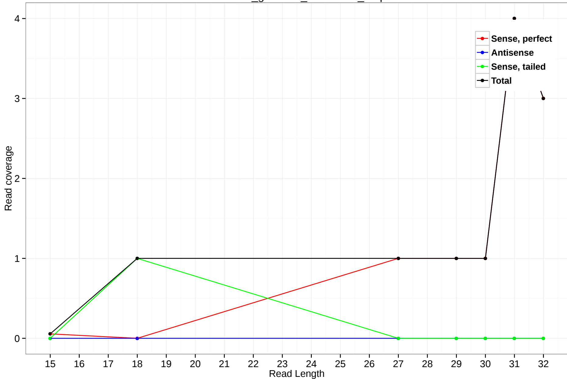
rheMac3_genscan_chr1.2738_6.3p
