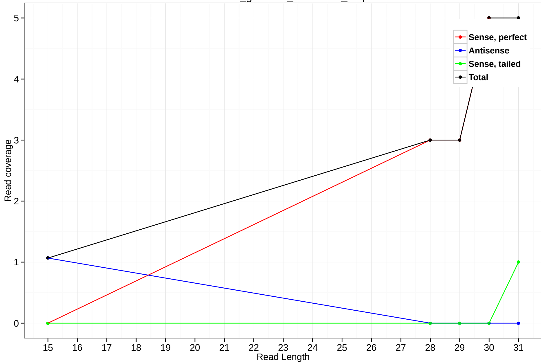
rheMac3_genscan_chr1.2738_2.5p
