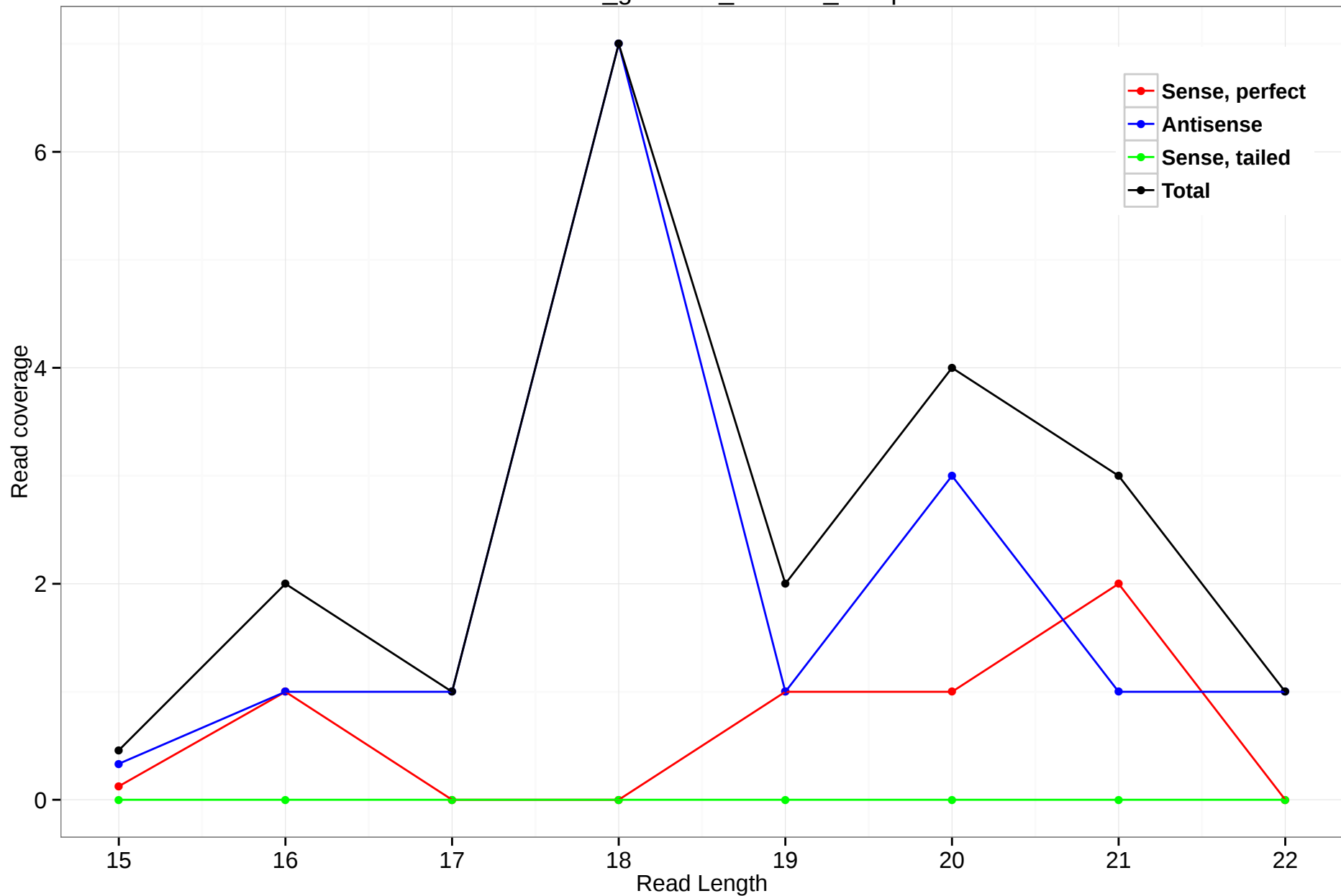
rheMac3_genscan_chr1.26_17.5p
