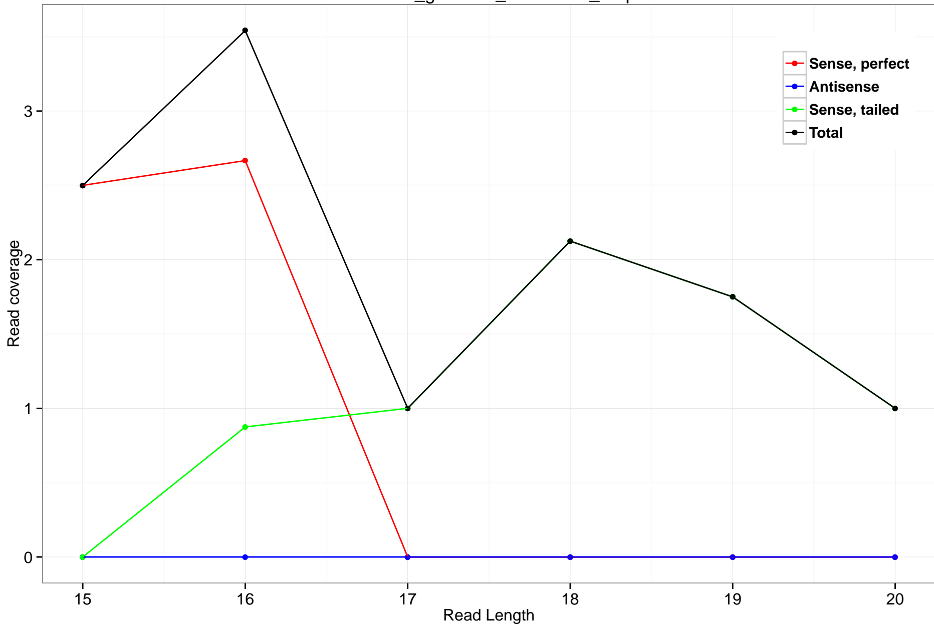
rheMac3_genscan_chr1.2647_4.3p
