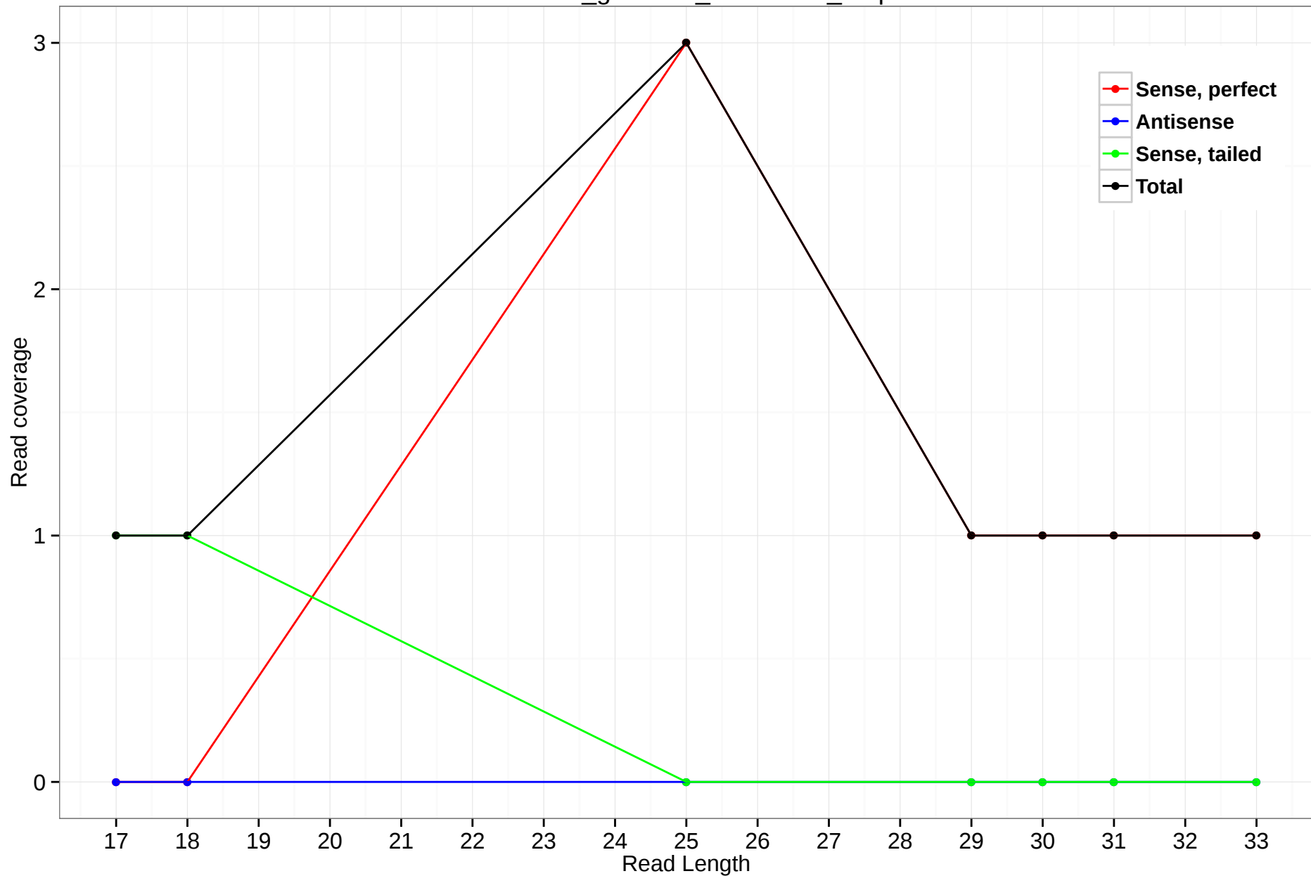
rheMac3_genscan_chr1.2637_2.3p
