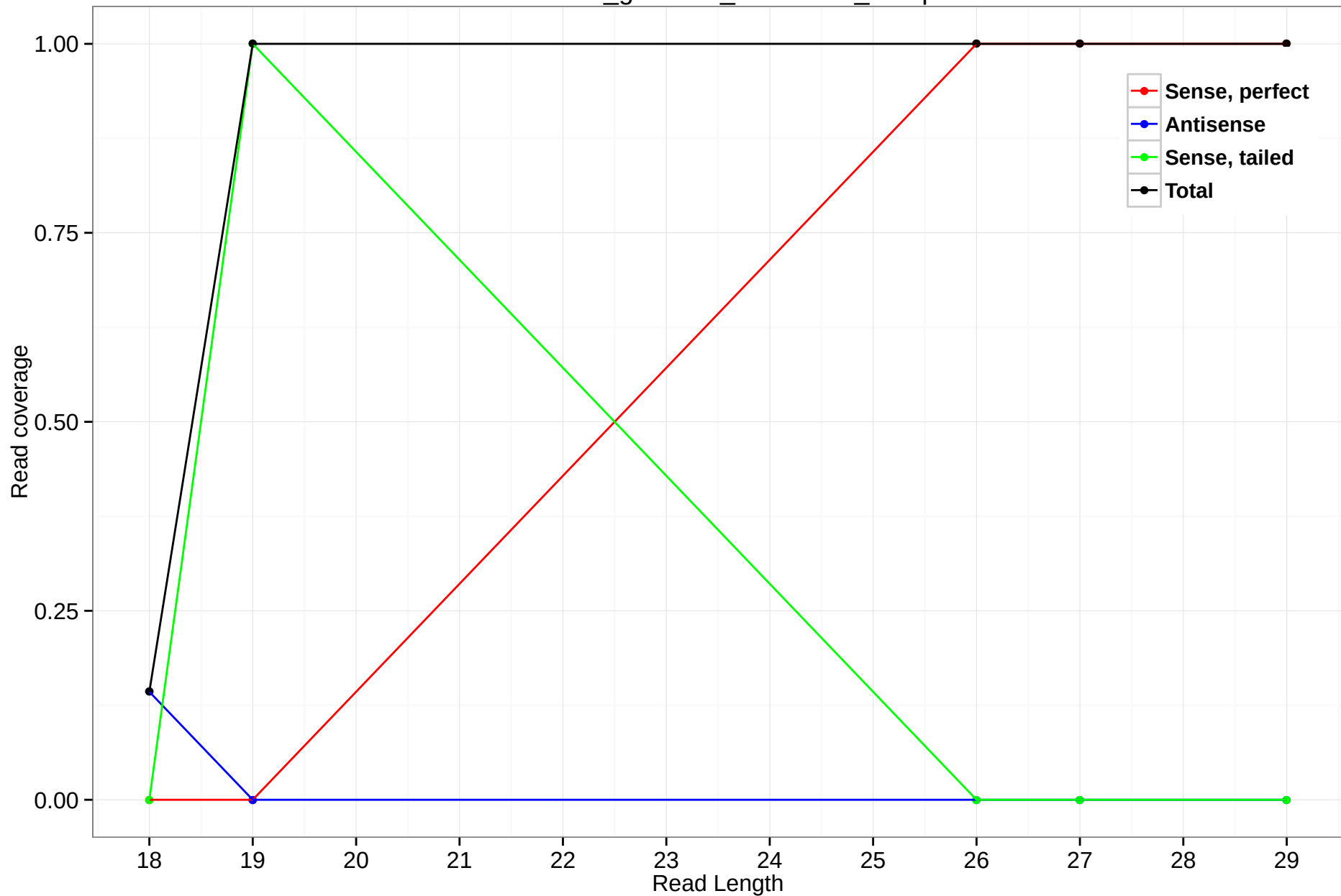
rheMac3_genscan_chr1.2629_15.3p
