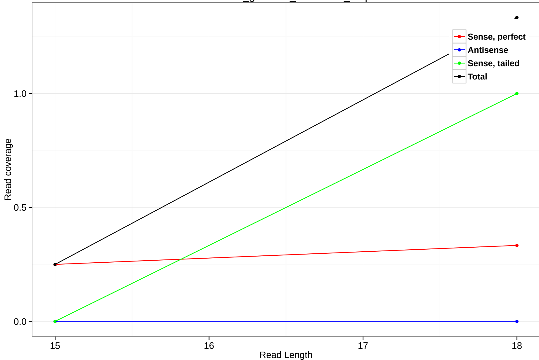
rheMac3_genscan_chr1.2576_3.3p
