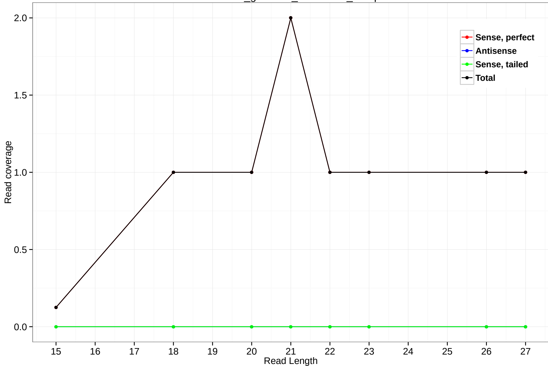
rheMac3_genscan_chr1.2574_12.5p
