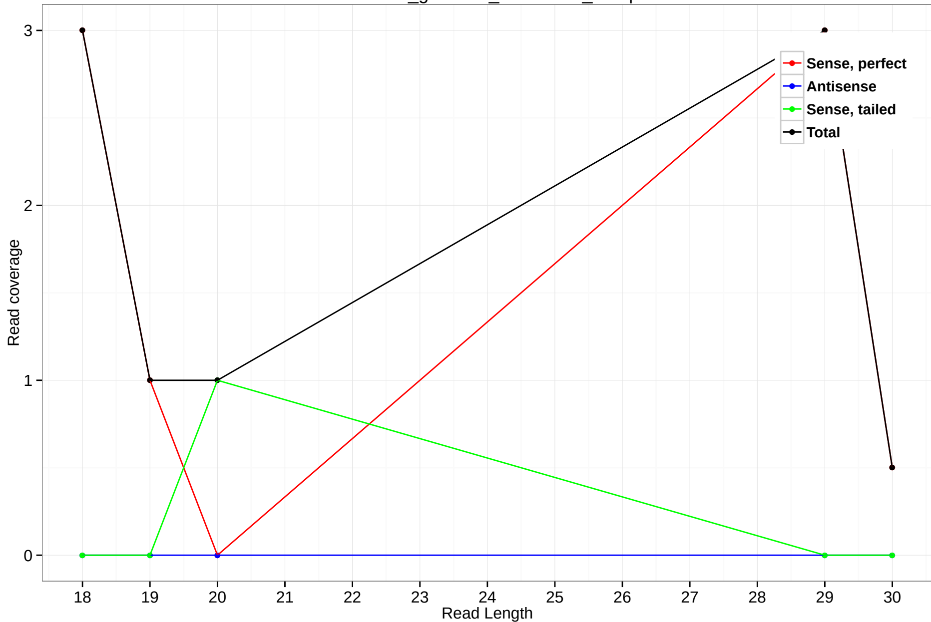
rheMac3_genscan_chr1.2542_11.5p
