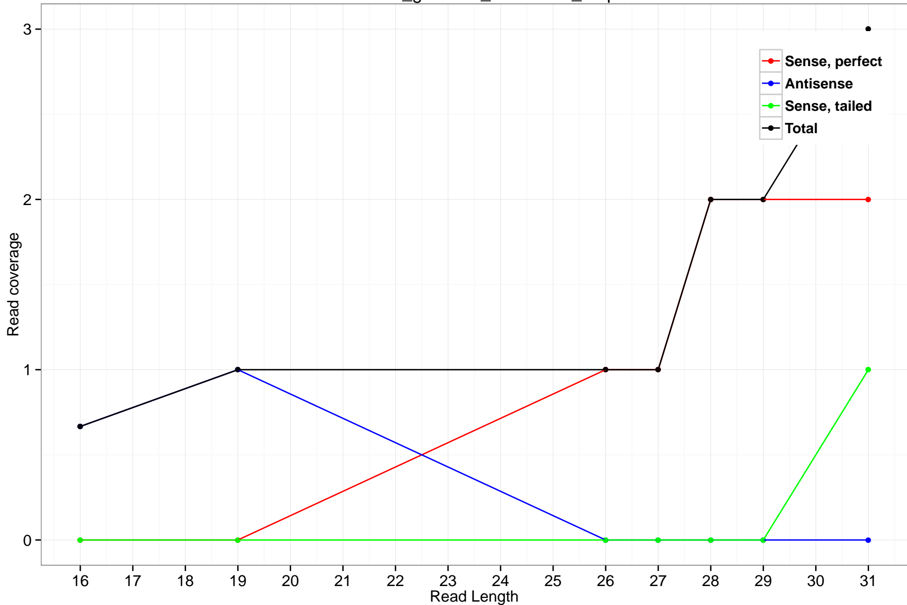
rheMac3_genscan_chr1.2538_0.3p
