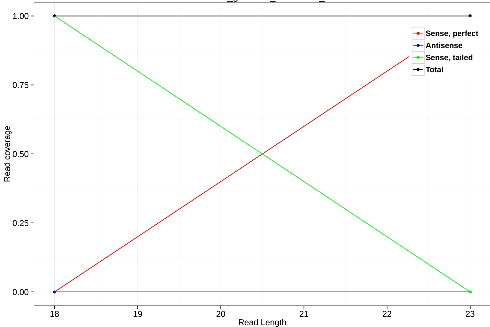
rheMac3_genscan_chr1.2496_43
