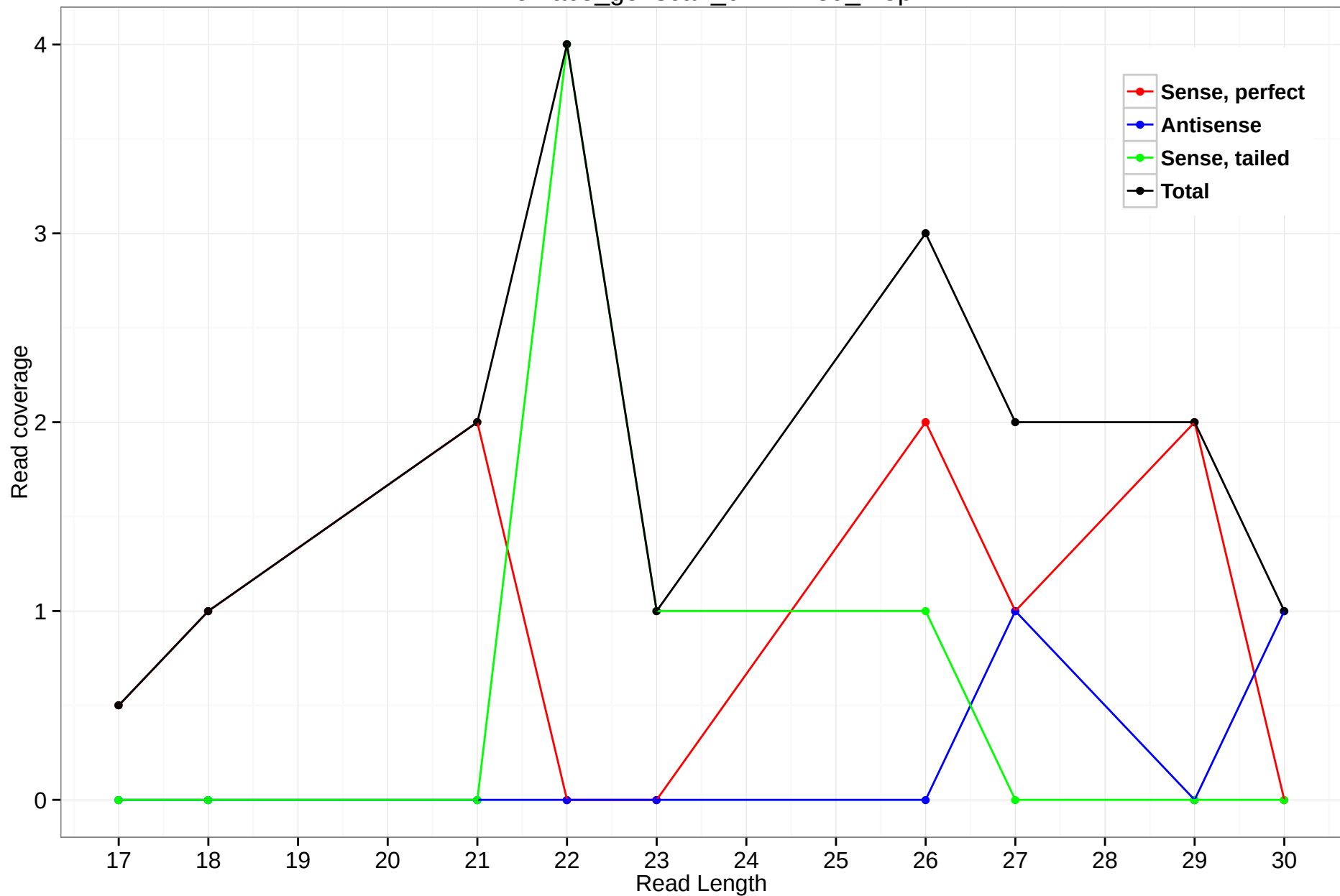
rheMac3_genscan_chr1.2489_1.3p
