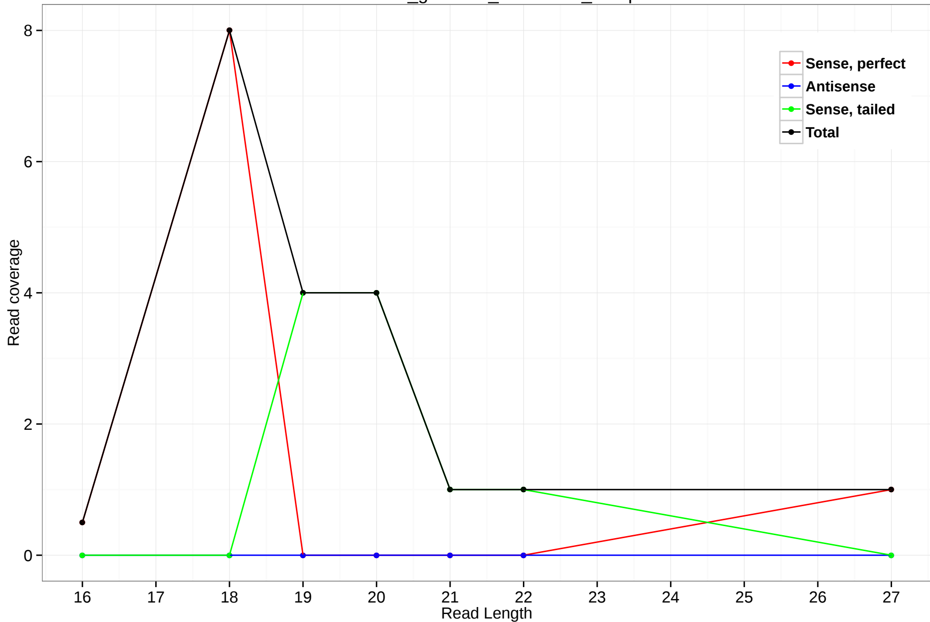
rheMac3_genscan_chr1.2486_33.3p
