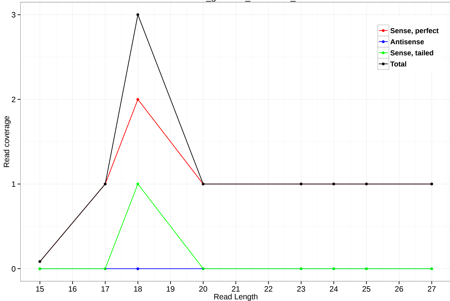
rheMac3_genscan_chr1.2420_2
