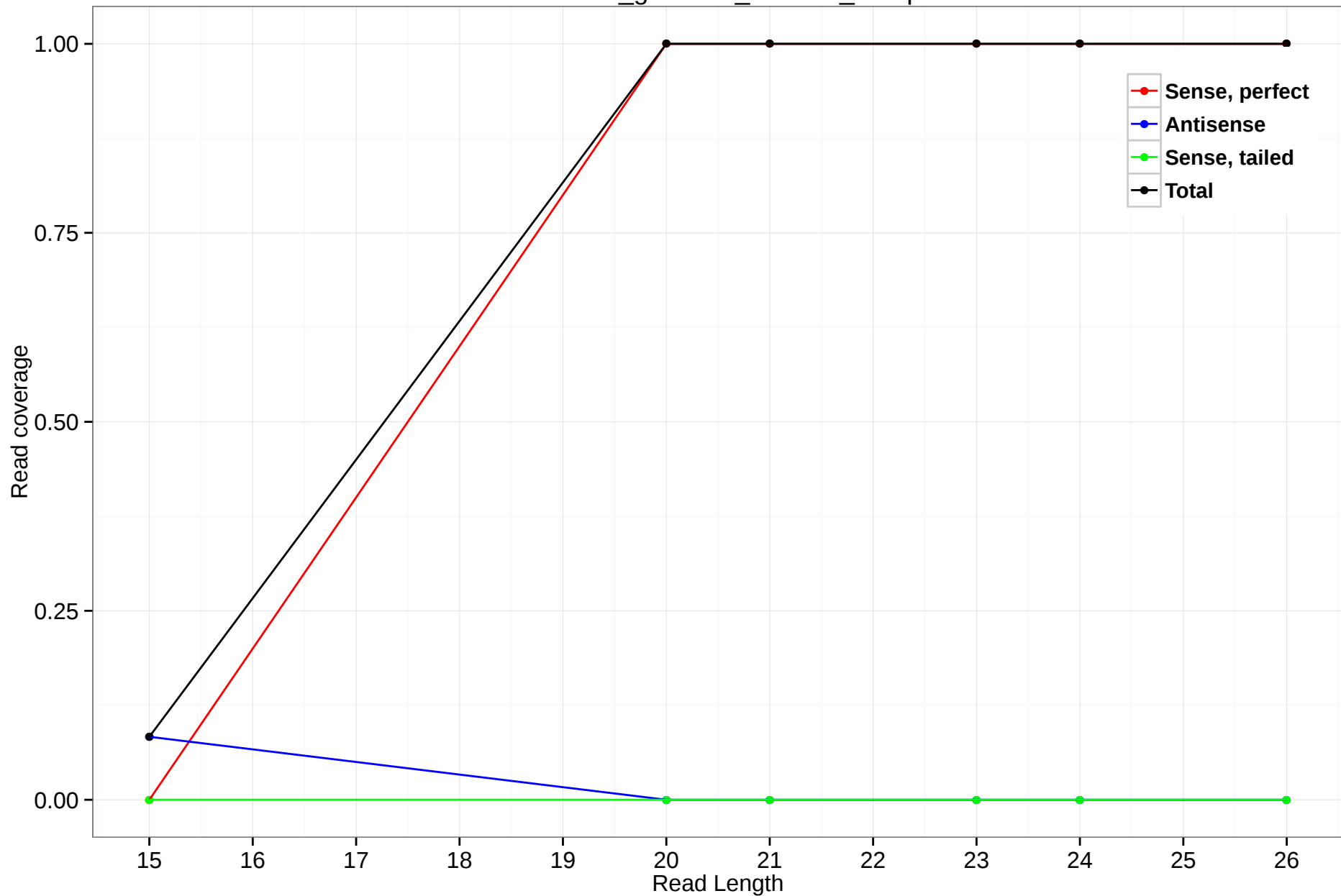
rheMac3_genscan_chr1.23_17.5p
