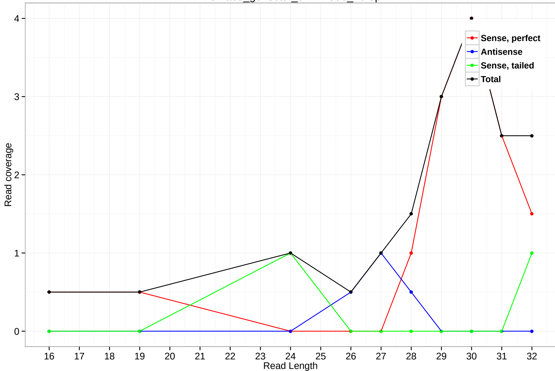
rheMac3_genscan_chr1.2306_20.5p
