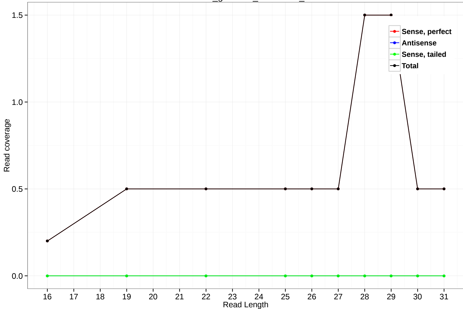
rheMac3_genscan_chr1.2306_18
