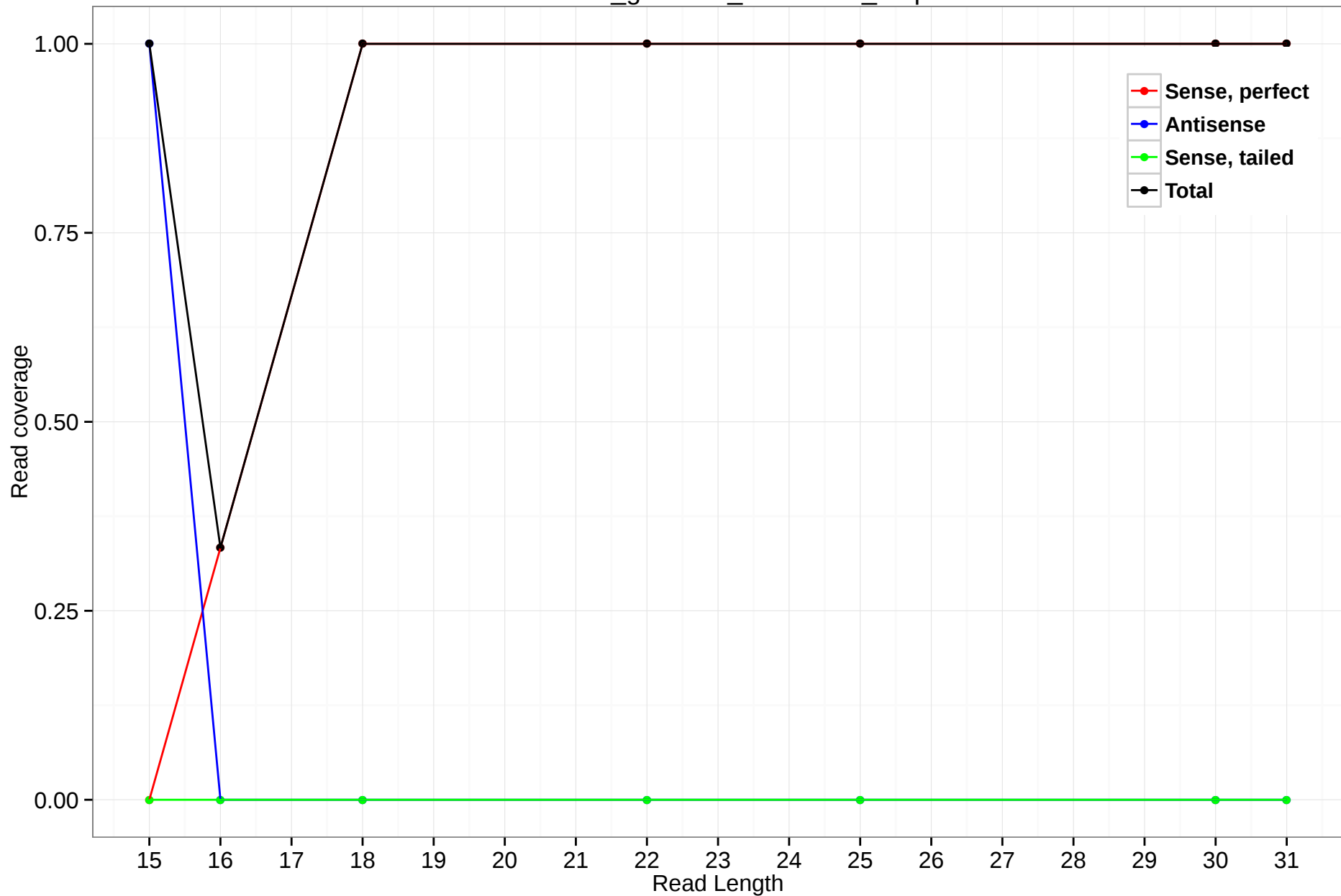
rheMac3_genscan_chr1.2295_7.5p
