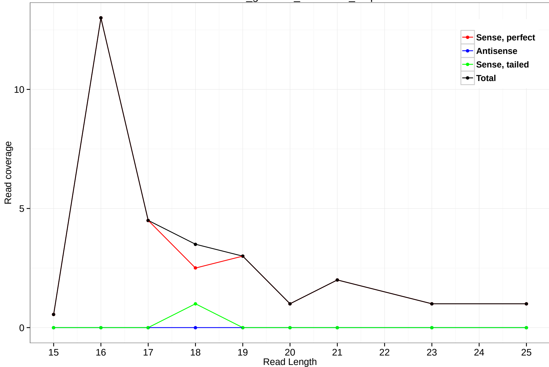
rheMac3_genscan_chr1.2295_2.3p
