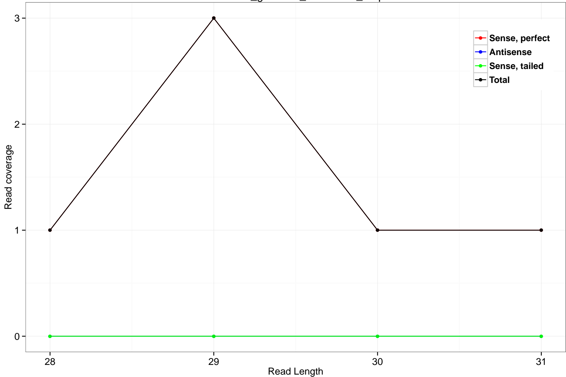
rheMac3_genscan_chr1.2289_5.3p
