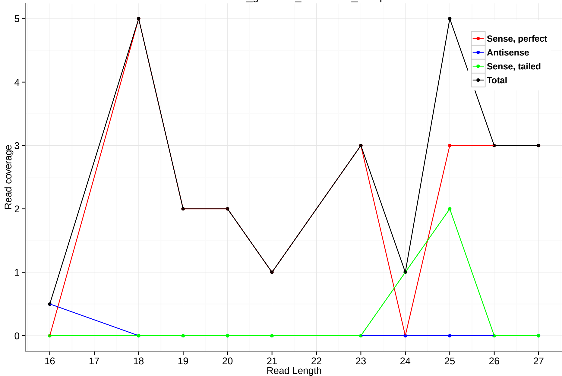
rheMac3_genscan_chr1.2221_16.3p
