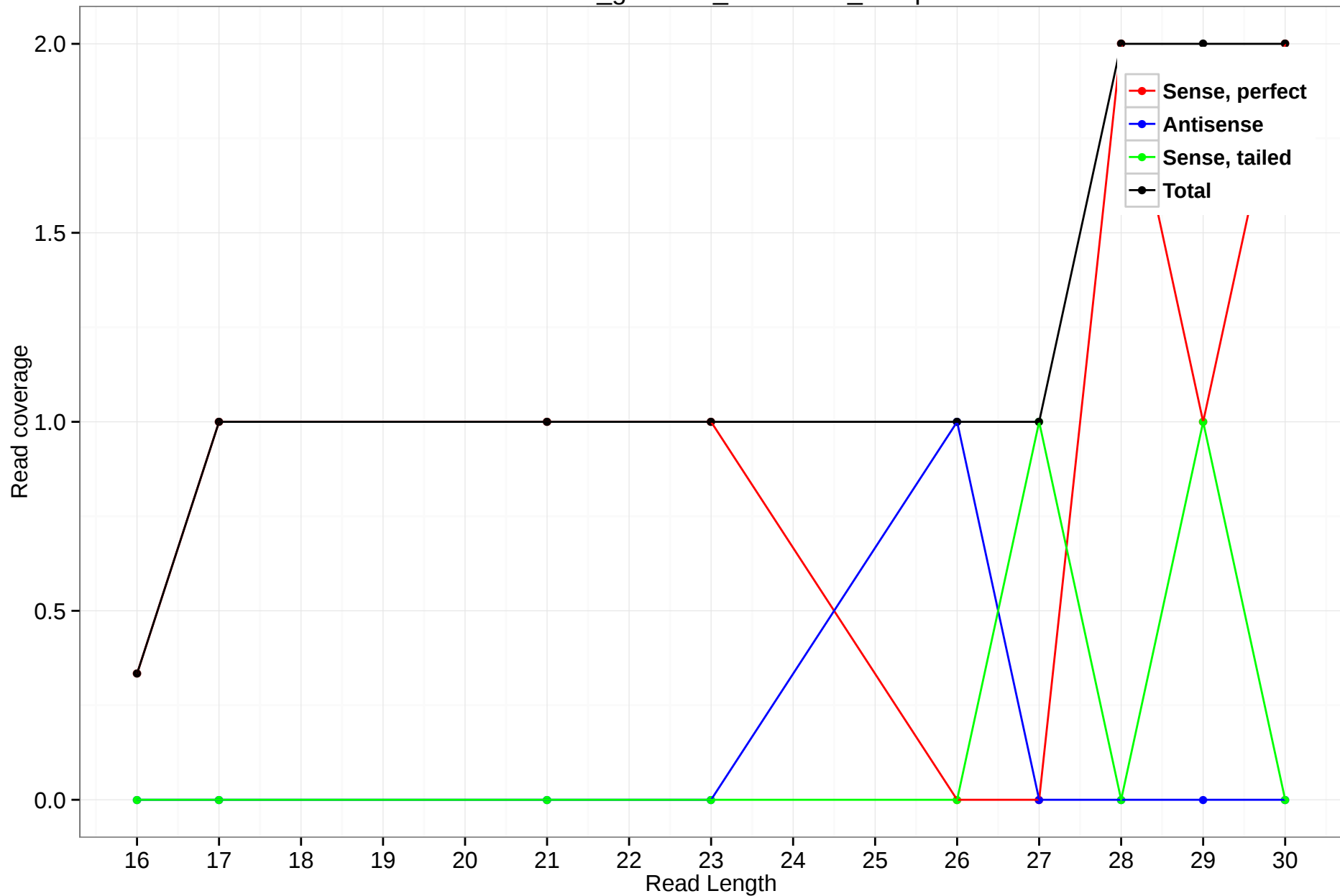
rheMac3_genscan_chr1.2209_25.3p
