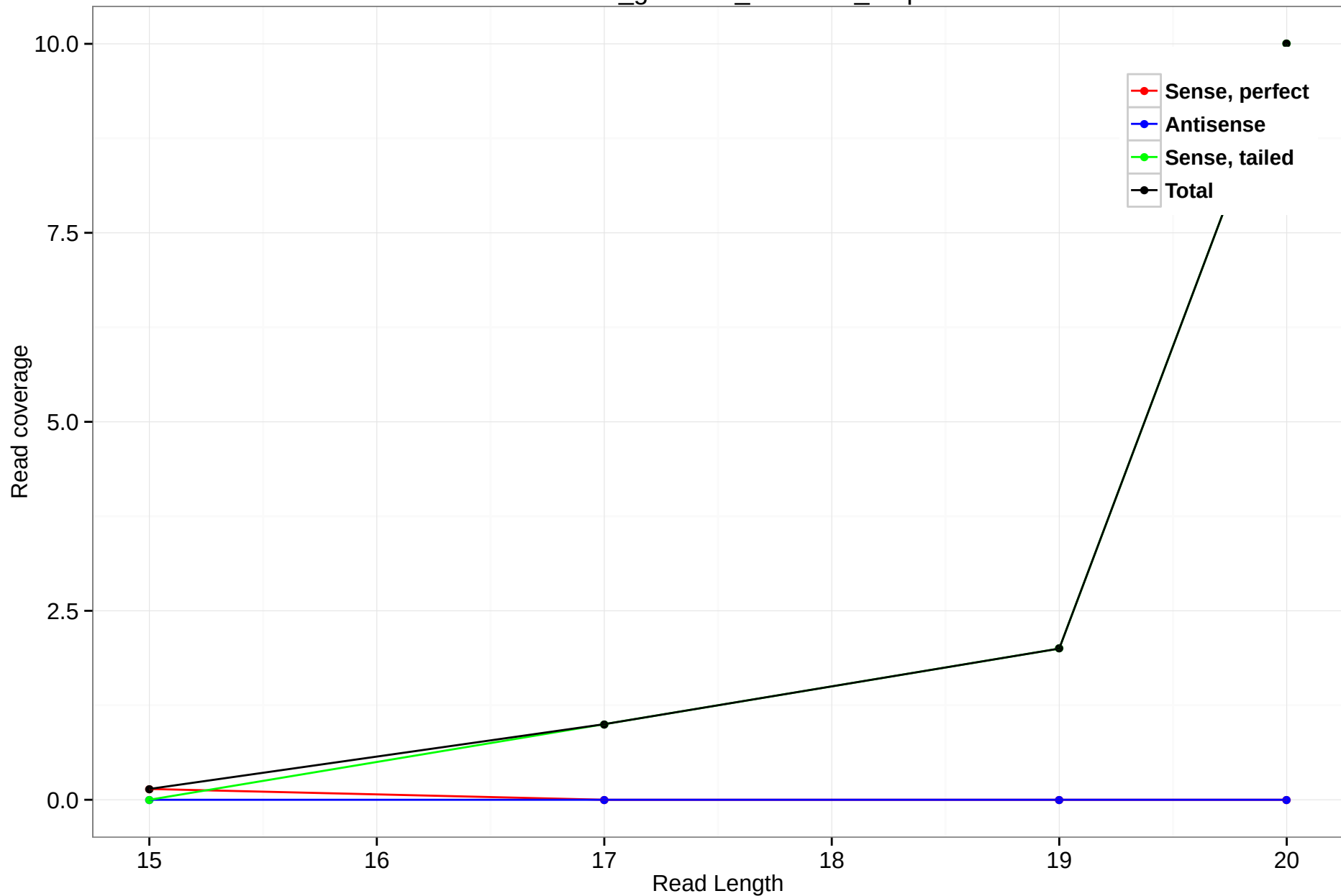
rheMac3_genscan_chr1.218_9.5p
