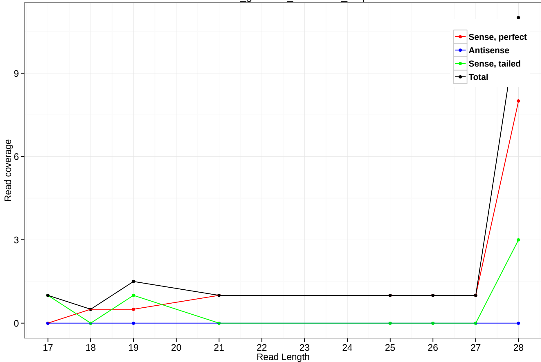
rheMac3_genscan_chr1.2120_0.3p
