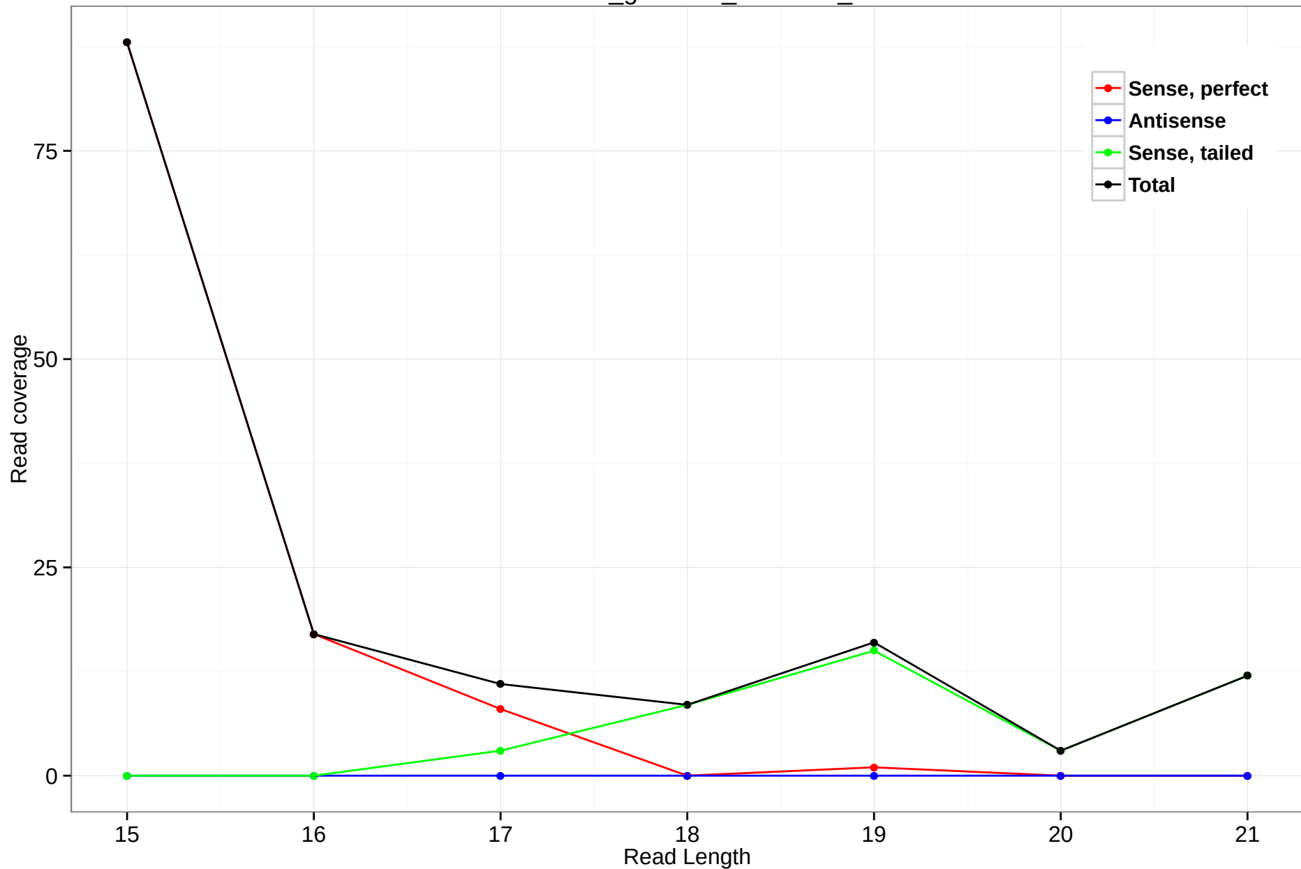
rheMac3_genscan_chr1.211_2
