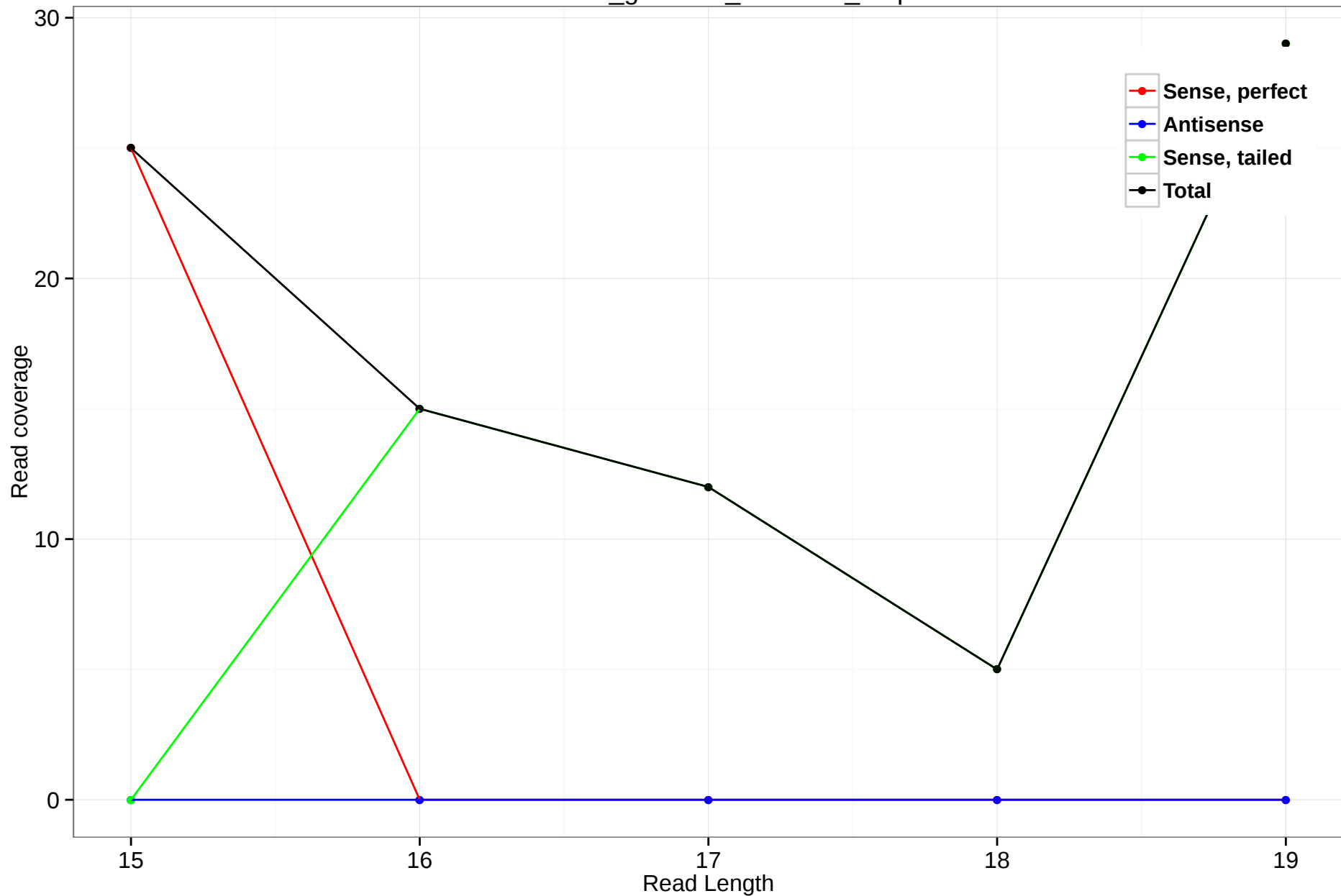
rheMac3_genscan_chr1.206_5.5p
