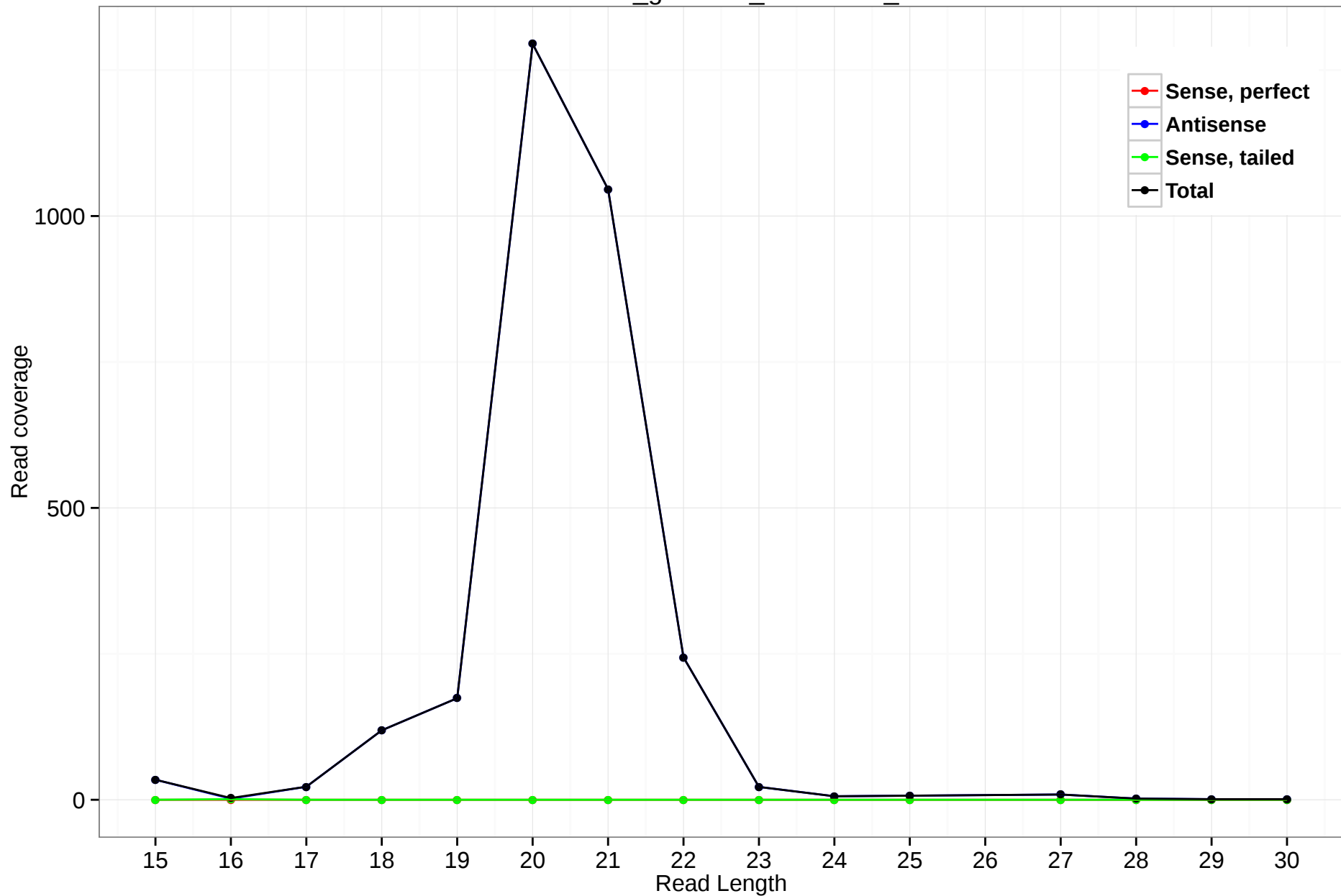
rheMac3_genscan_chr1.1993_7
