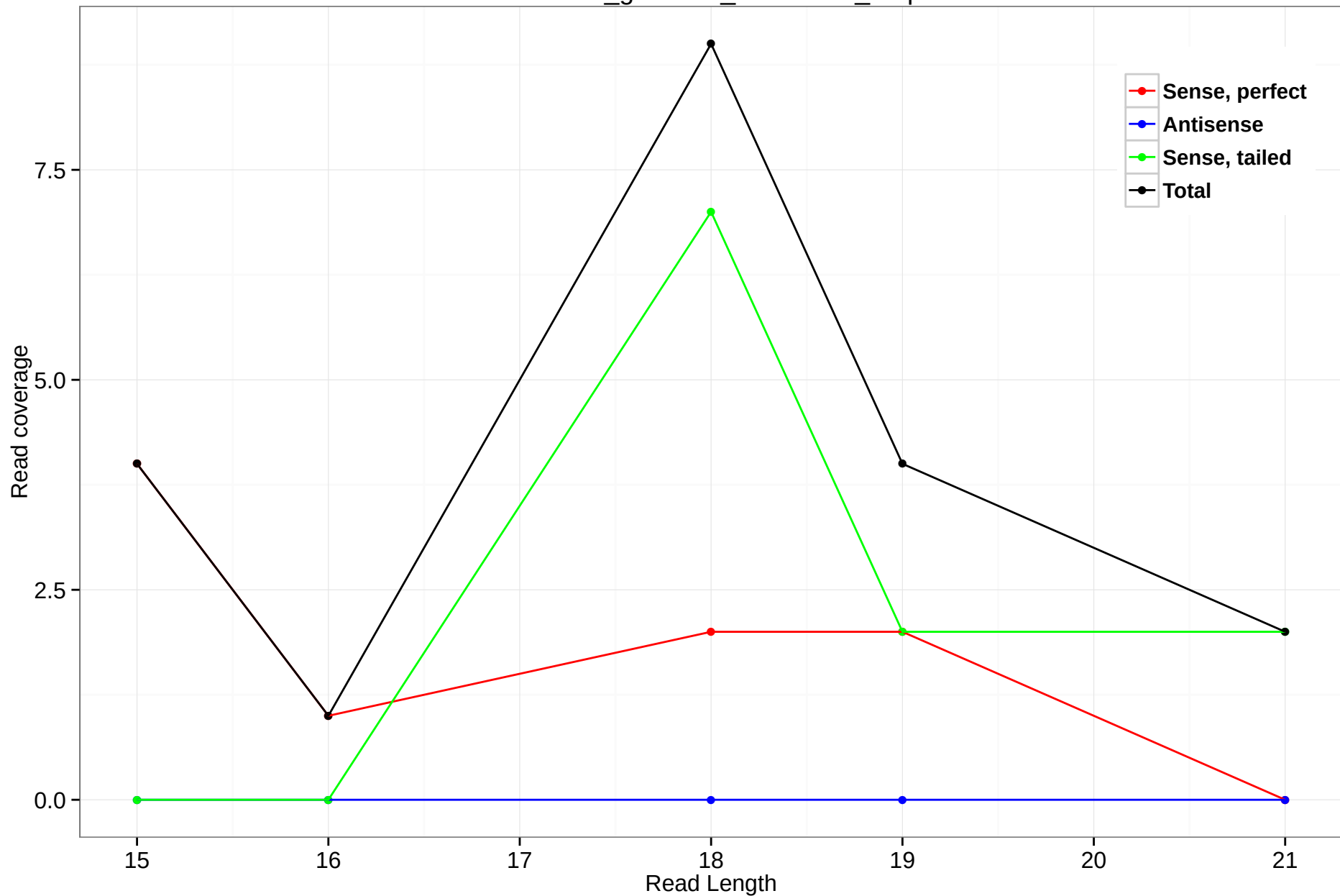
rheMac3_genscan_chr1.1947_3.3p
