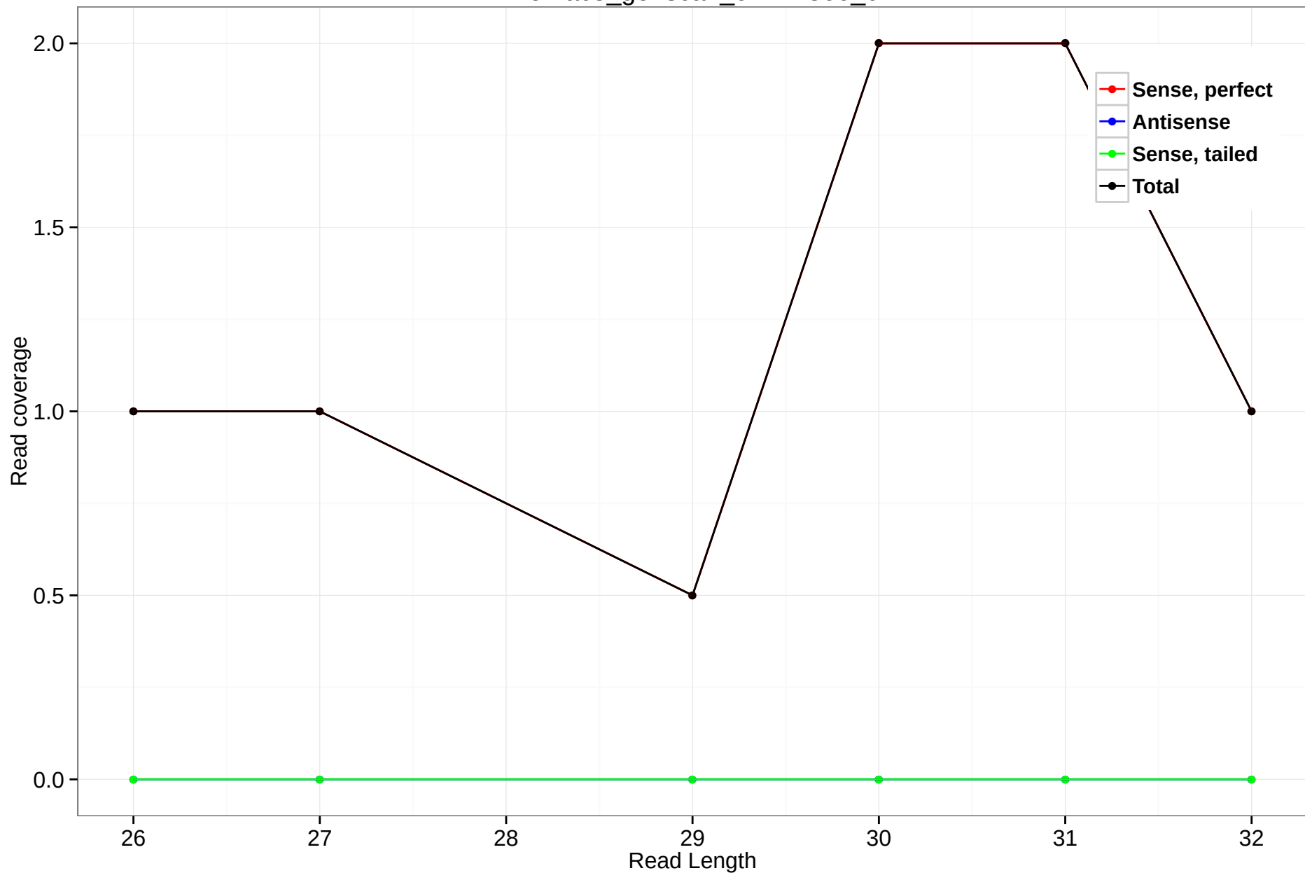
rheMac3_genscan_chr1.1866_0
