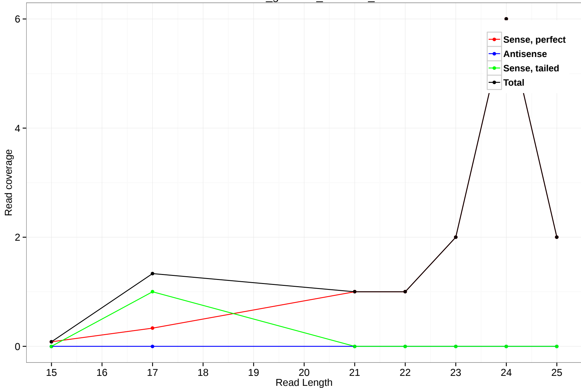
rheMac3_genscan_chr1.181_16
