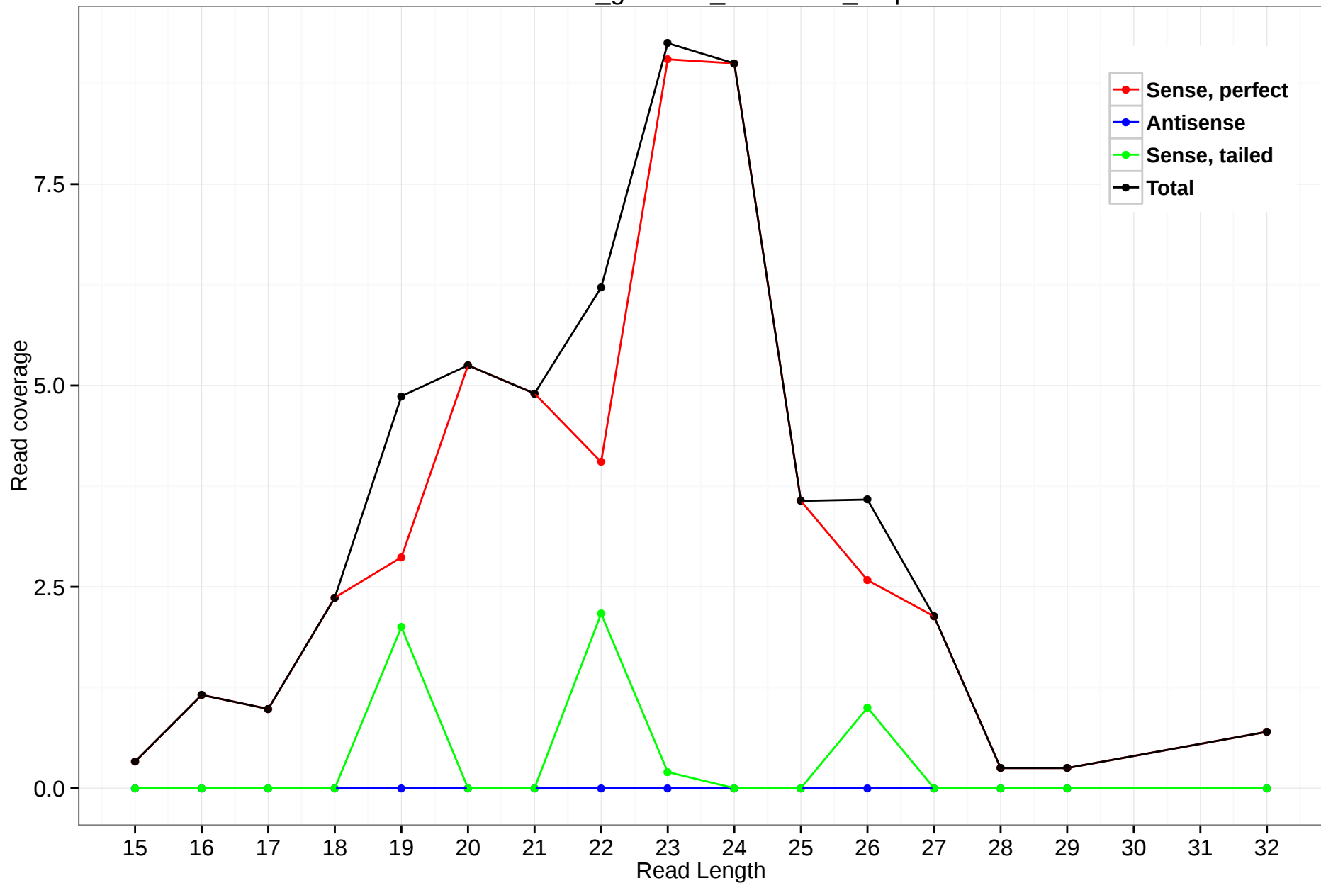
rheMac3_genscan_chr1.1762_1.3p
